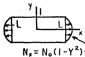
Fig 5. Full Plate Convergence Study With Parabolic Tension End Condition
