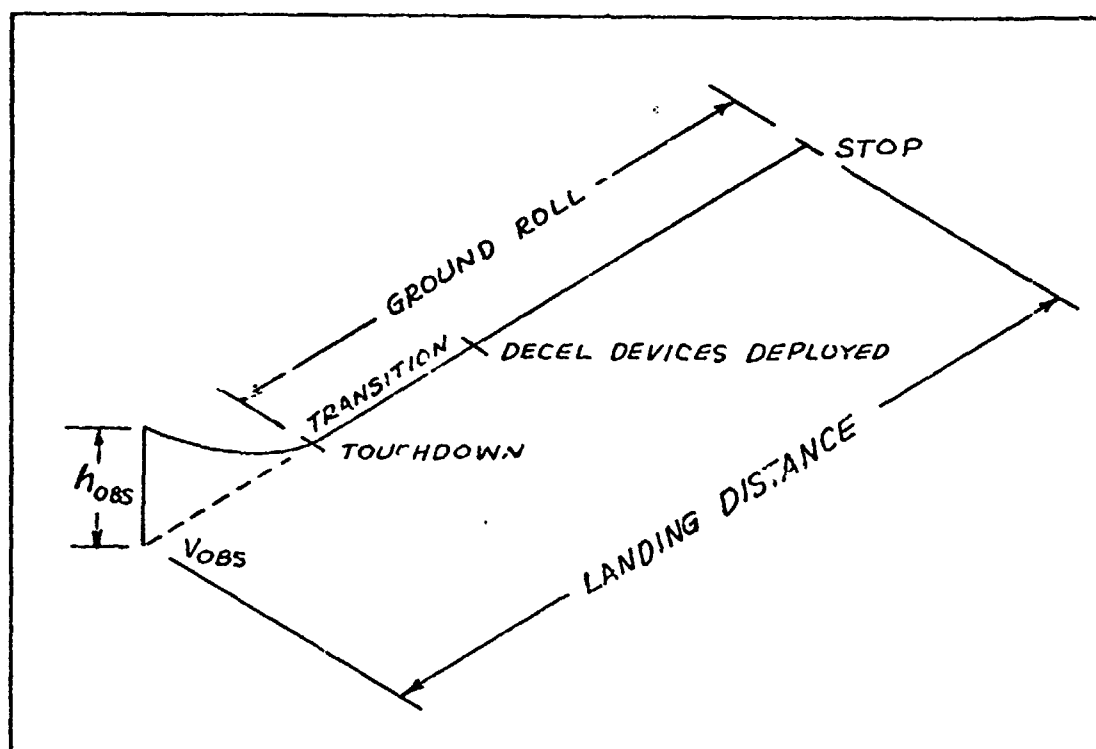
Figure 3. Landing Distance Schematic
