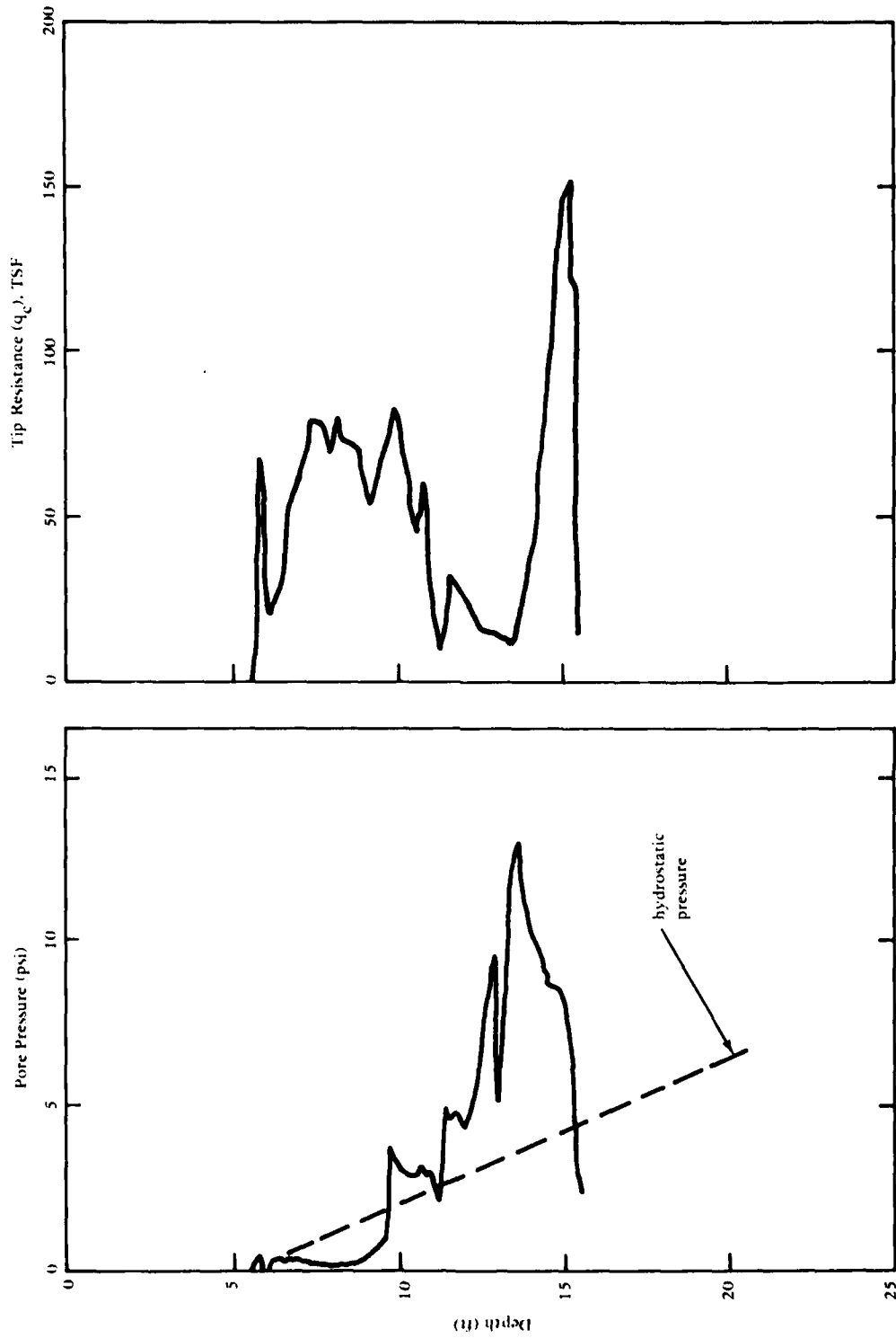
Figure 7. Piezometer sounding.
