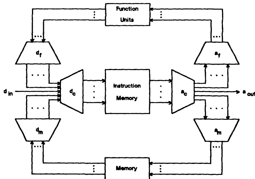
Figure C.1 The routing networks
