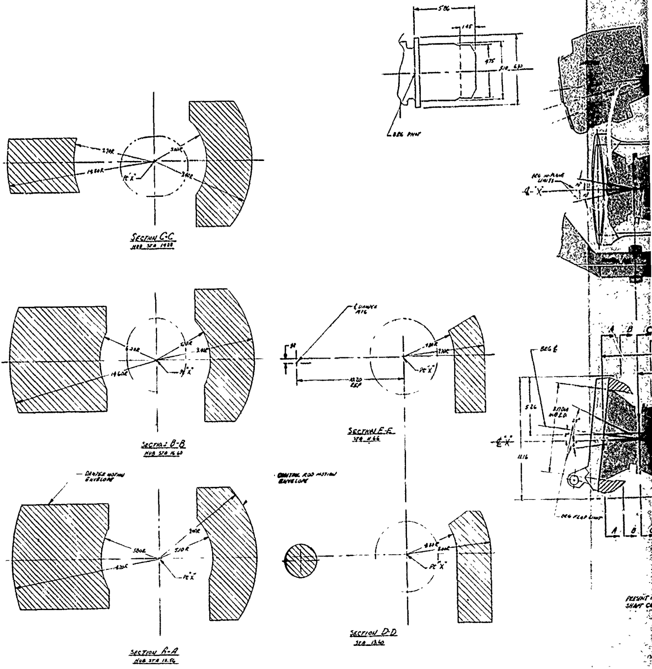
FIGURE 3 GEOMETRIC REQUIREMENTS FOR UH-60A ROTOR HUB
