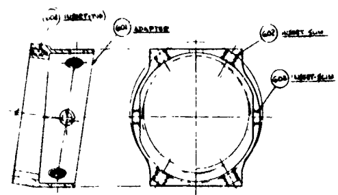
(040) DETL C BEARING RING (SEE SECTION B-B)
