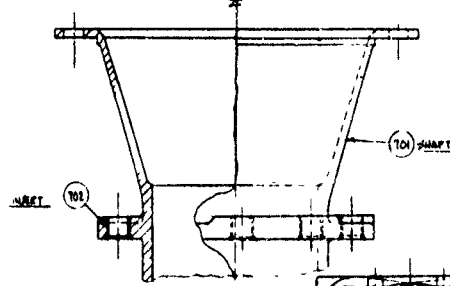
(07) SHAFT DETL G
