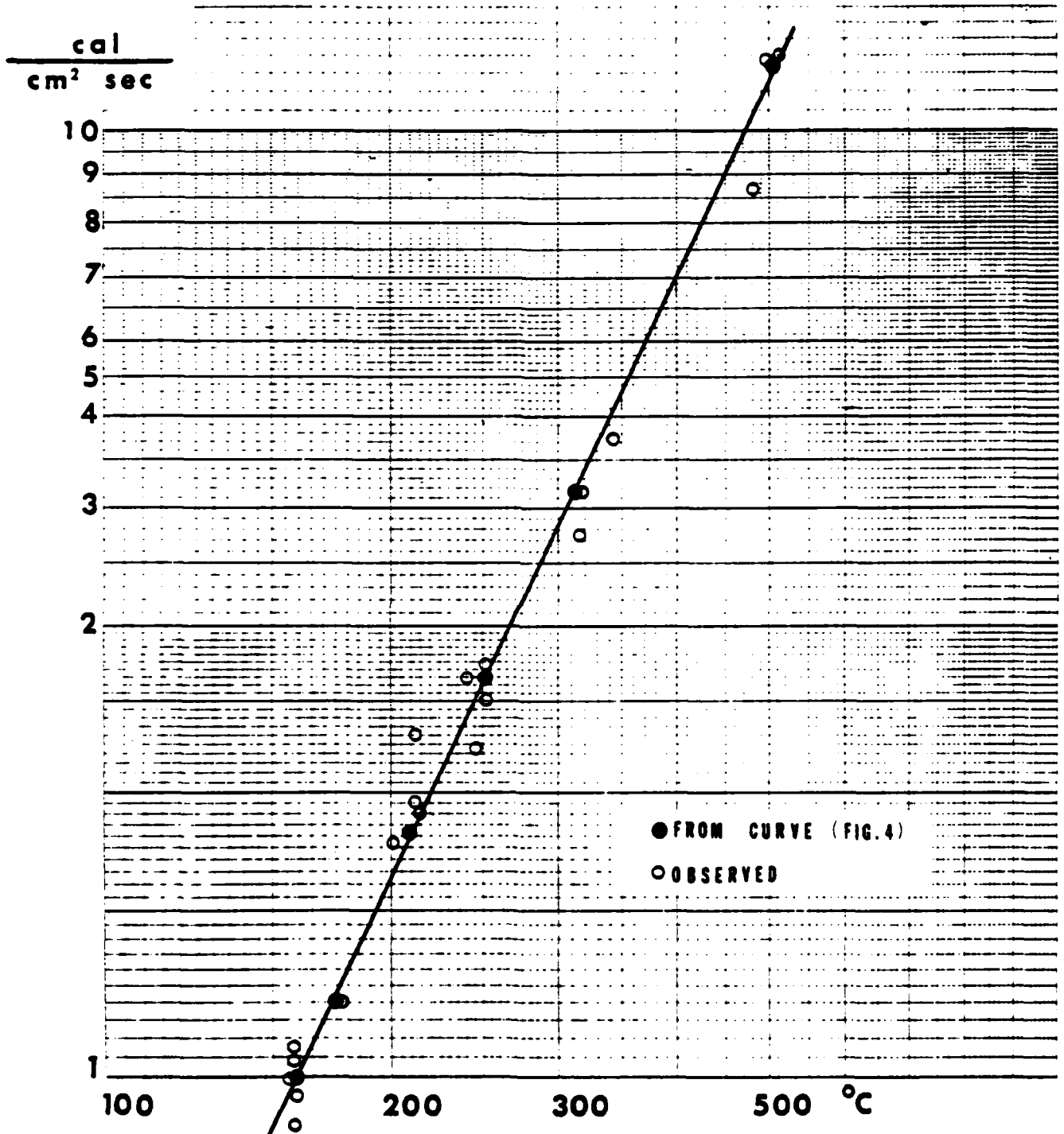
Flame Temperature as Indicated by #30 Gauge Thermocouple at 1 Second
