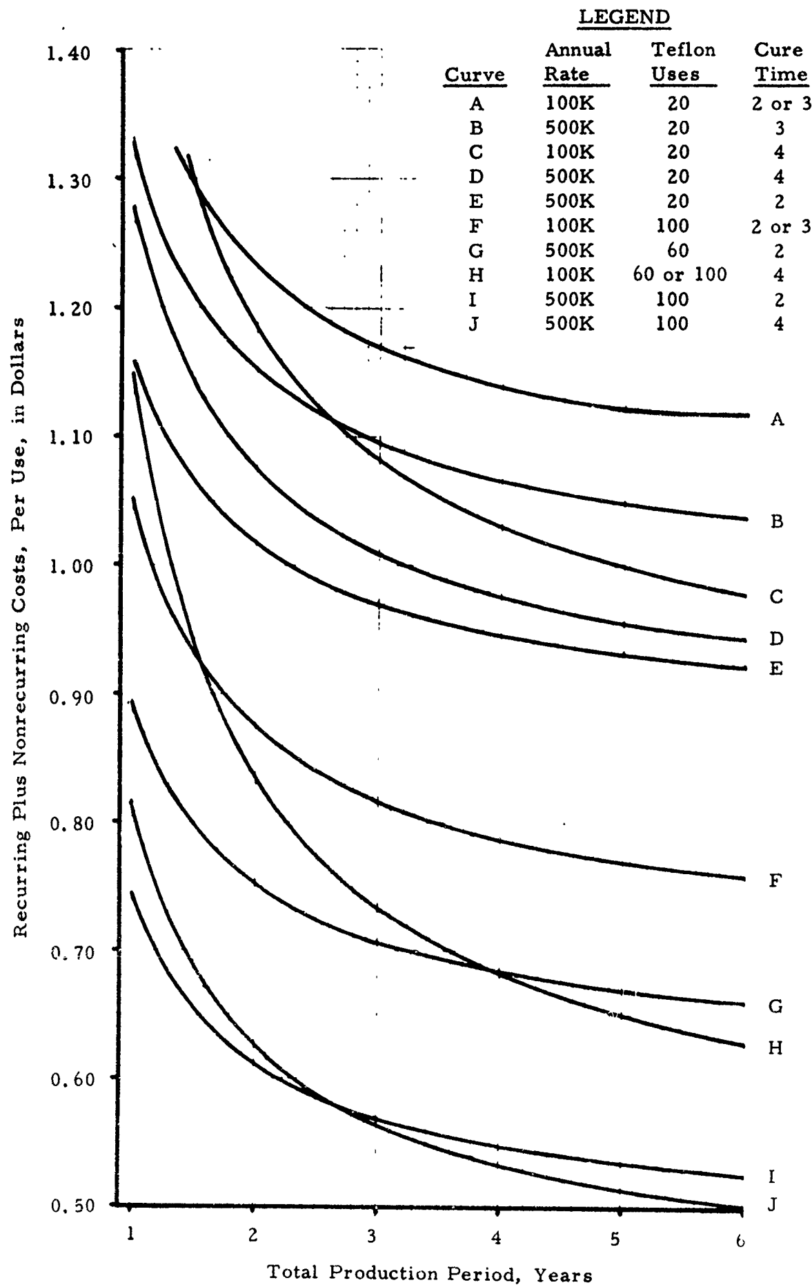
Figure 70. Net Per Use Cost, Typical Curves, Viper Reusable Tooling Concept
