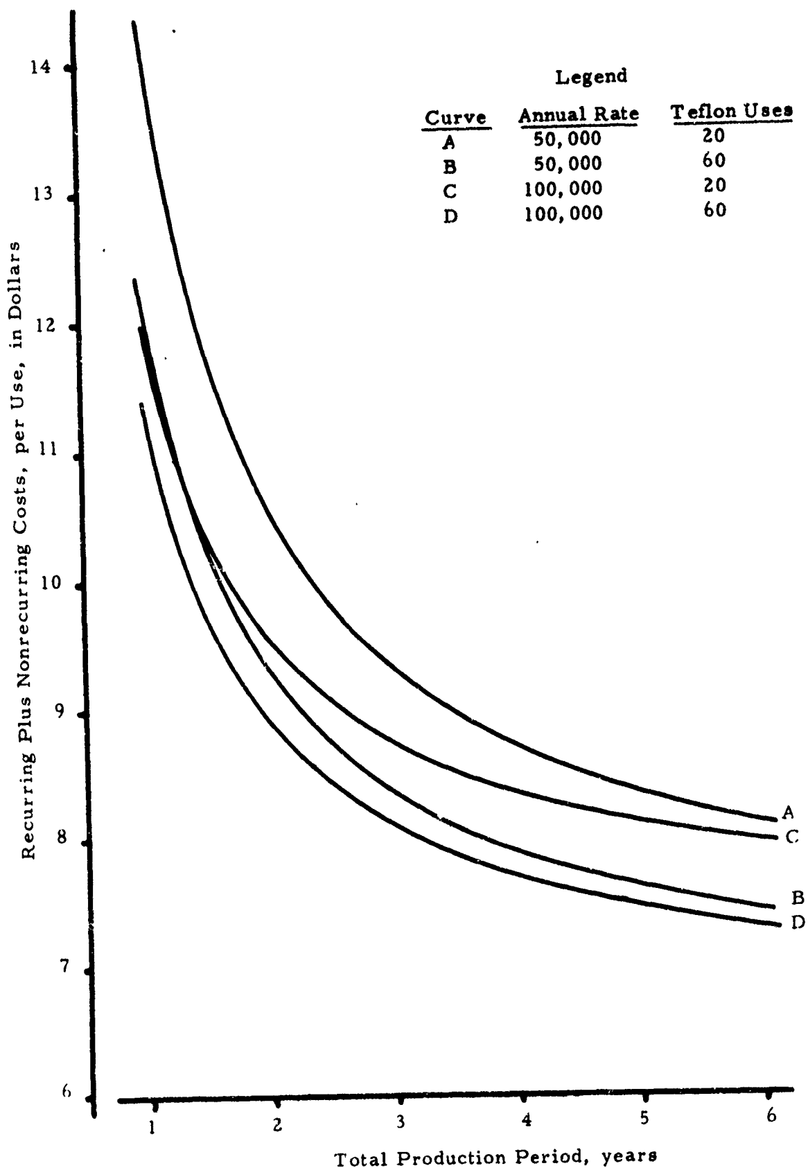
Figure 86. Net Per Use Cost, FFR Reusable Tooling
