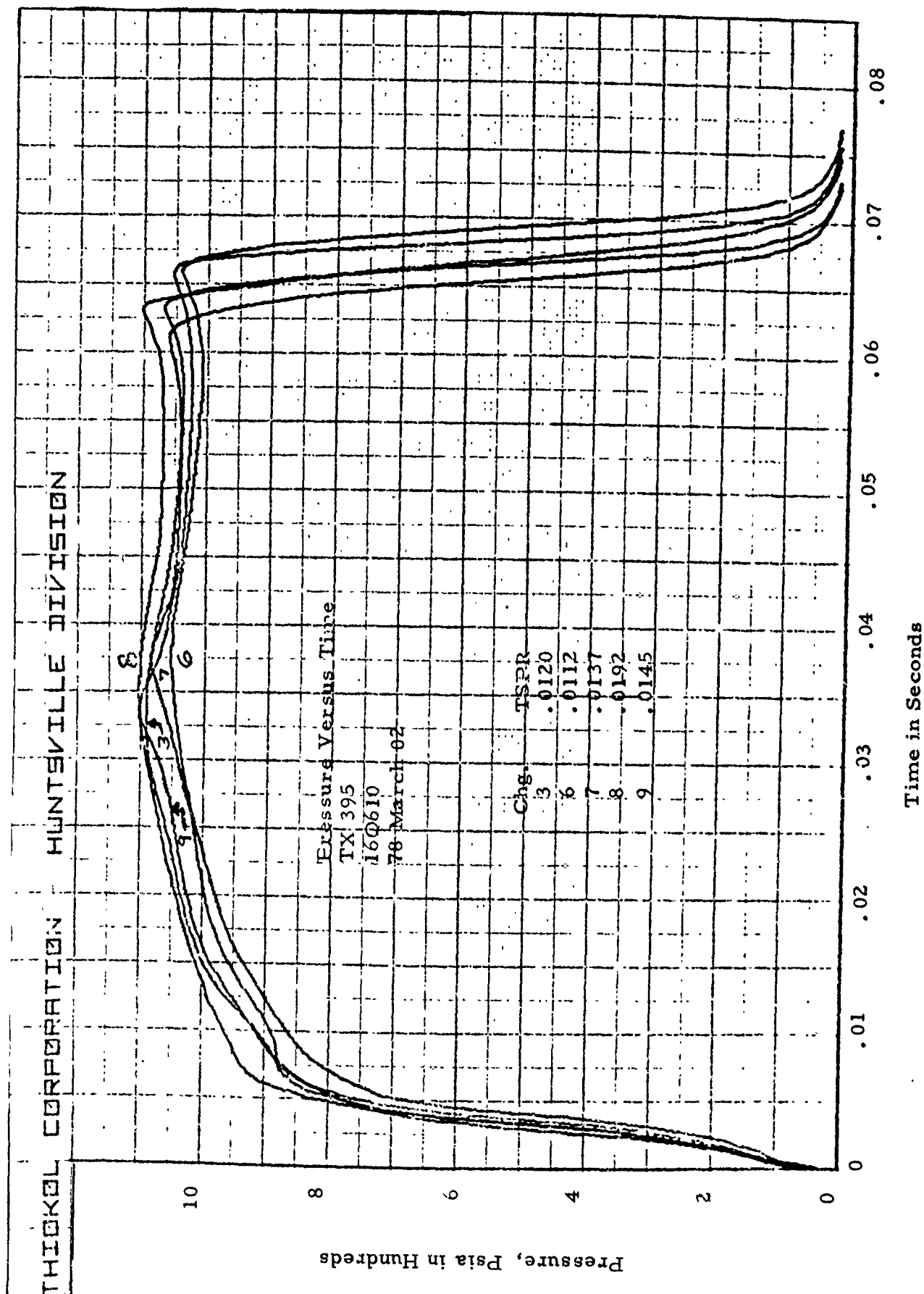
Figure 13. Mandrel Pull Test Ballistic Data SEAS Propellant (16Q610-3, -6, -7, -8, -9)
