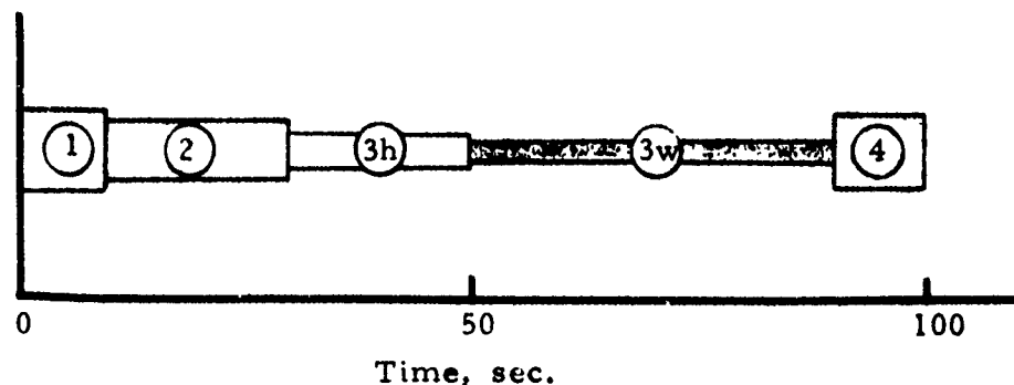
Figure 44. Typical Thermoset Molding Cycles (1) Press Closing; (2) flow period (including degassing when used); (3w) Cure Time Without Preheat; and (4) Press Opening.
