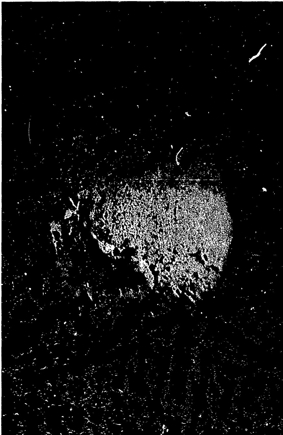
Figure 31. Surface Formed by PTMT Core in SEAS-type Propellant, Motor 16Q-610-2
