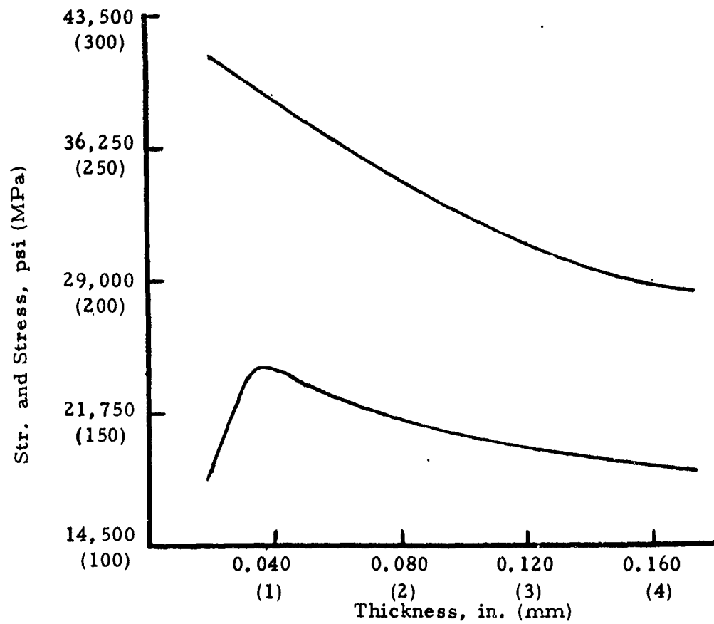
Figure 38. Ultimate Tensile Strength and Proof Strength as They Relate to Casting Wall Thickness*
