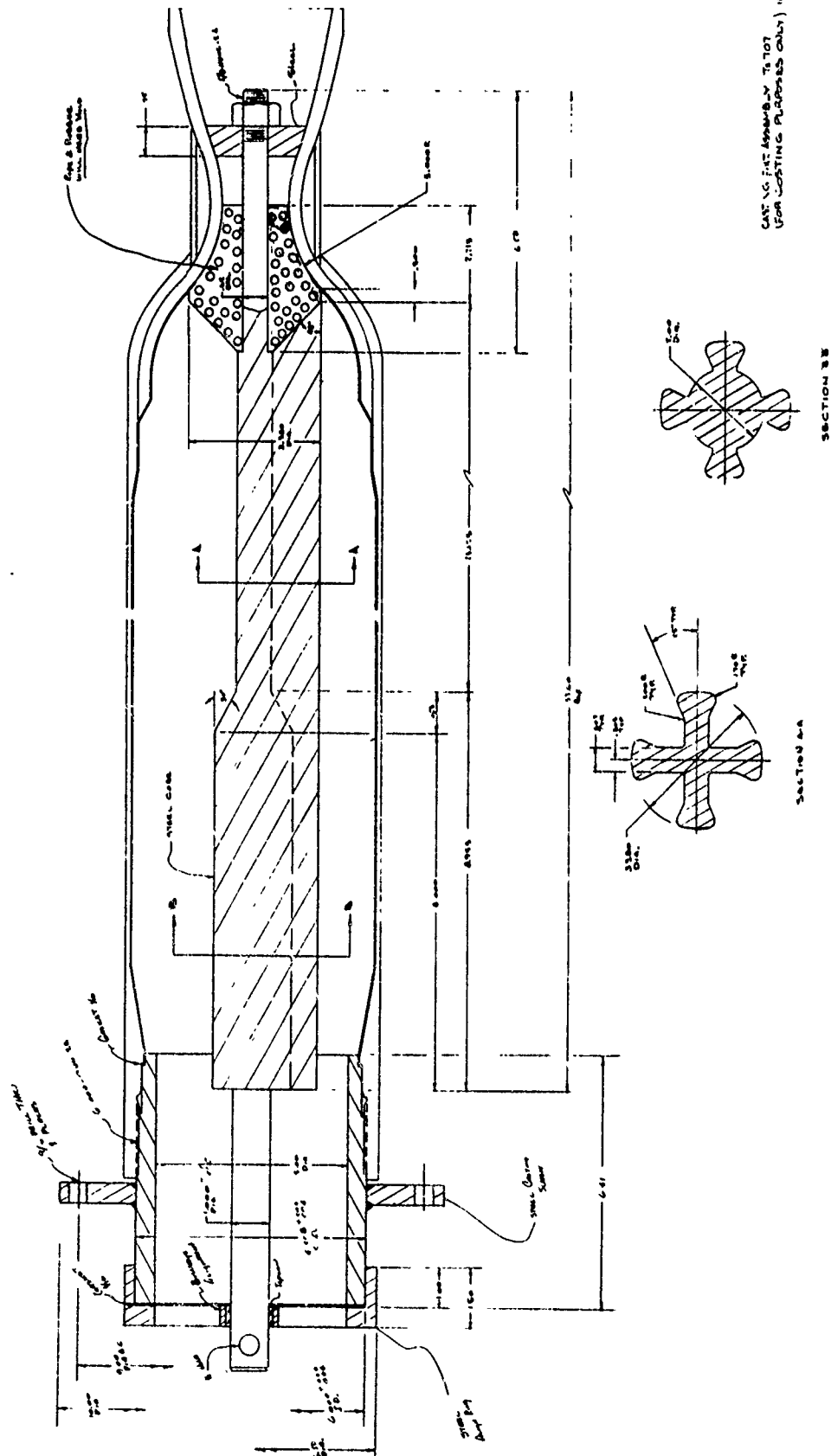
Figure 84. Removable Metal Mandrel for TX707 FFR Motor.
