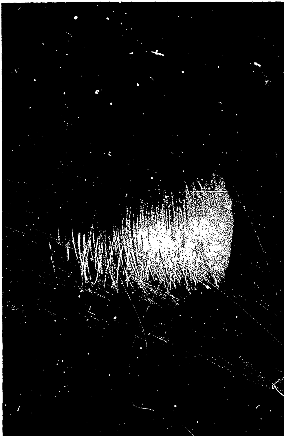
Figure 23. Surface Formed by Polypropylene Core in SEAS-type Propellant Motor 16Q-609-2
