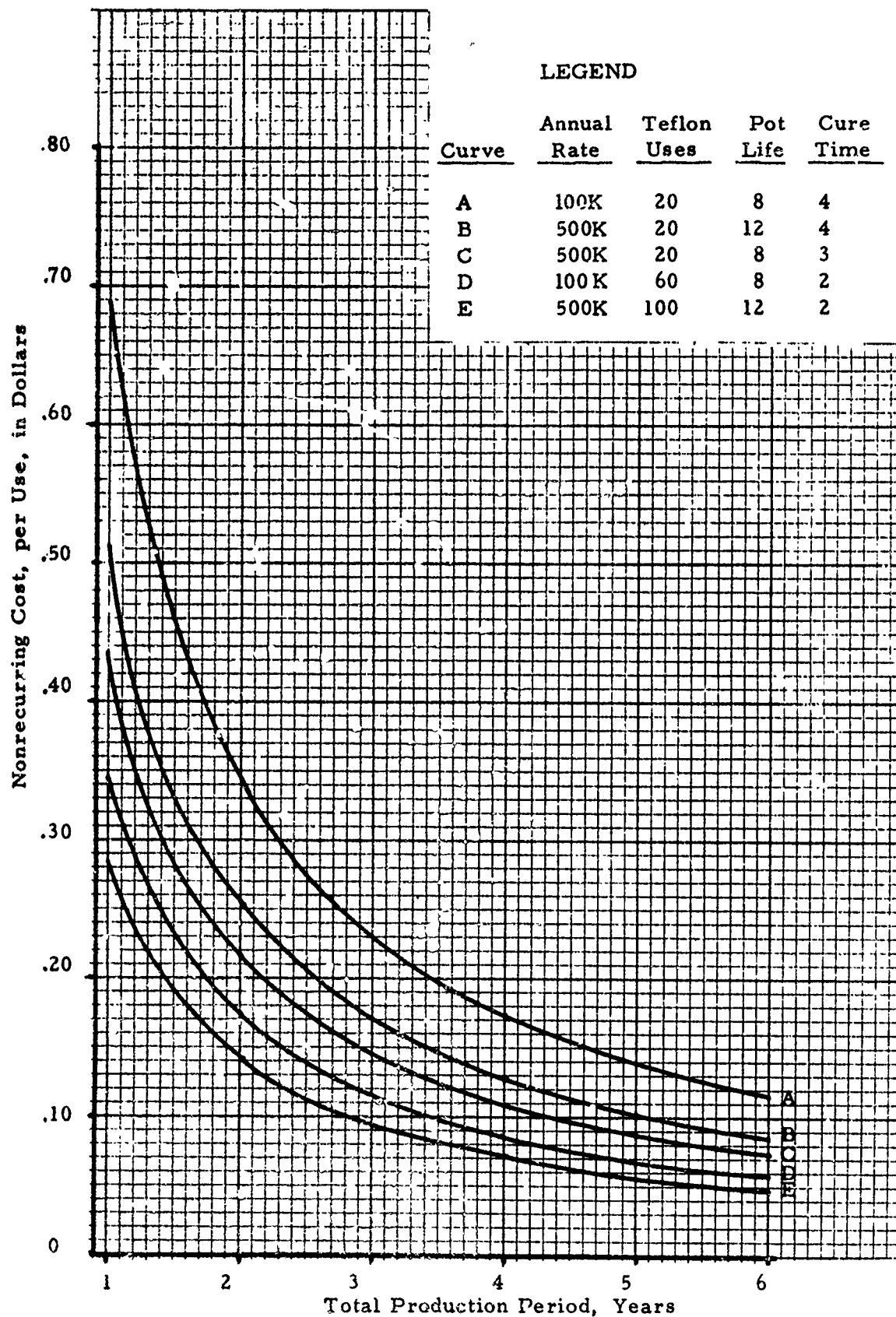
Figure 60. Nonrecurring Costs per Use, Typical Curves
