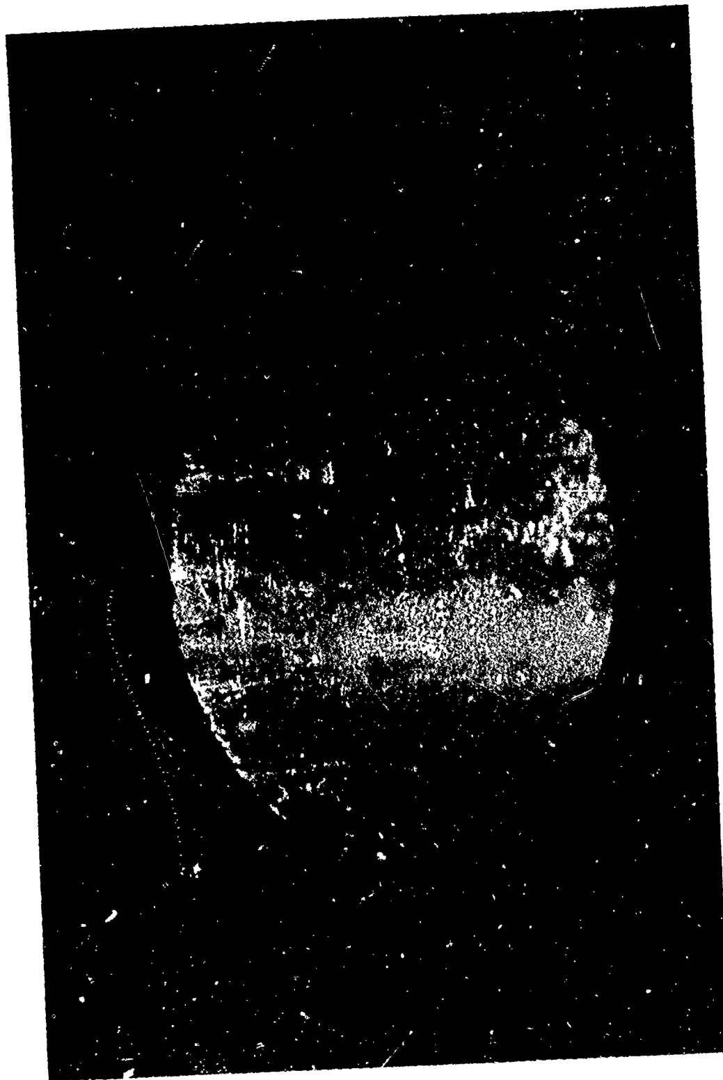
Figure 19. Surface Formed by Teflon-coated Steel Core, Sprayed with IMS, in Viper Propellant, Motor 16Q-607-8
