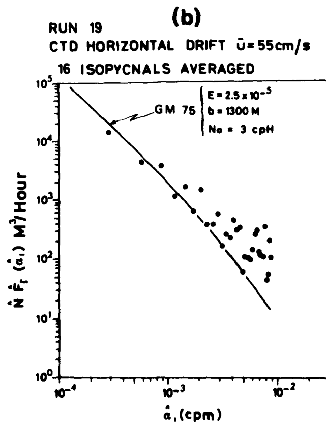
FIG. 12 SPECTRAL ANALYSIS OF HORIZONTAL TEMPERATURE CHANGES
