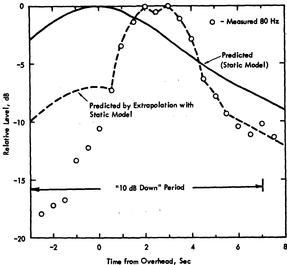
Figure 12. Comparison of Measured Time History of Relative One-Third Octave Band Level at 80 Hz from 727 on Takeoff with Values Predicted by Simple "Static" Model for Moving Monopole Source (Directivity, Kinematic and Acoustic Effects of Motion Ignored). Dashed Lines Designate Predicted Values when Levels Less than 10 dB Below Maximum Must Be Estimated by Using Temporal Extrapolation Based on a Static Model for the Change in Propagation Loss with Time. (Aircraft Altitude 244 m, Speed = 80 m/s, Mach No. = 0.23, Atmospheric Attenuation Coefficient = 0.013 dB/100 m)
