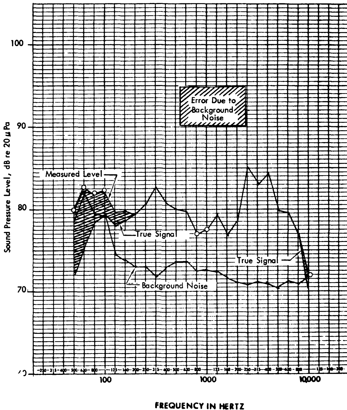
Figure 18. 727 Approach with Background Noise Raised to Create Seven Bands in Violation of 5 dB Requirement. Bands with o are Within 5 dB of Background Noise.
