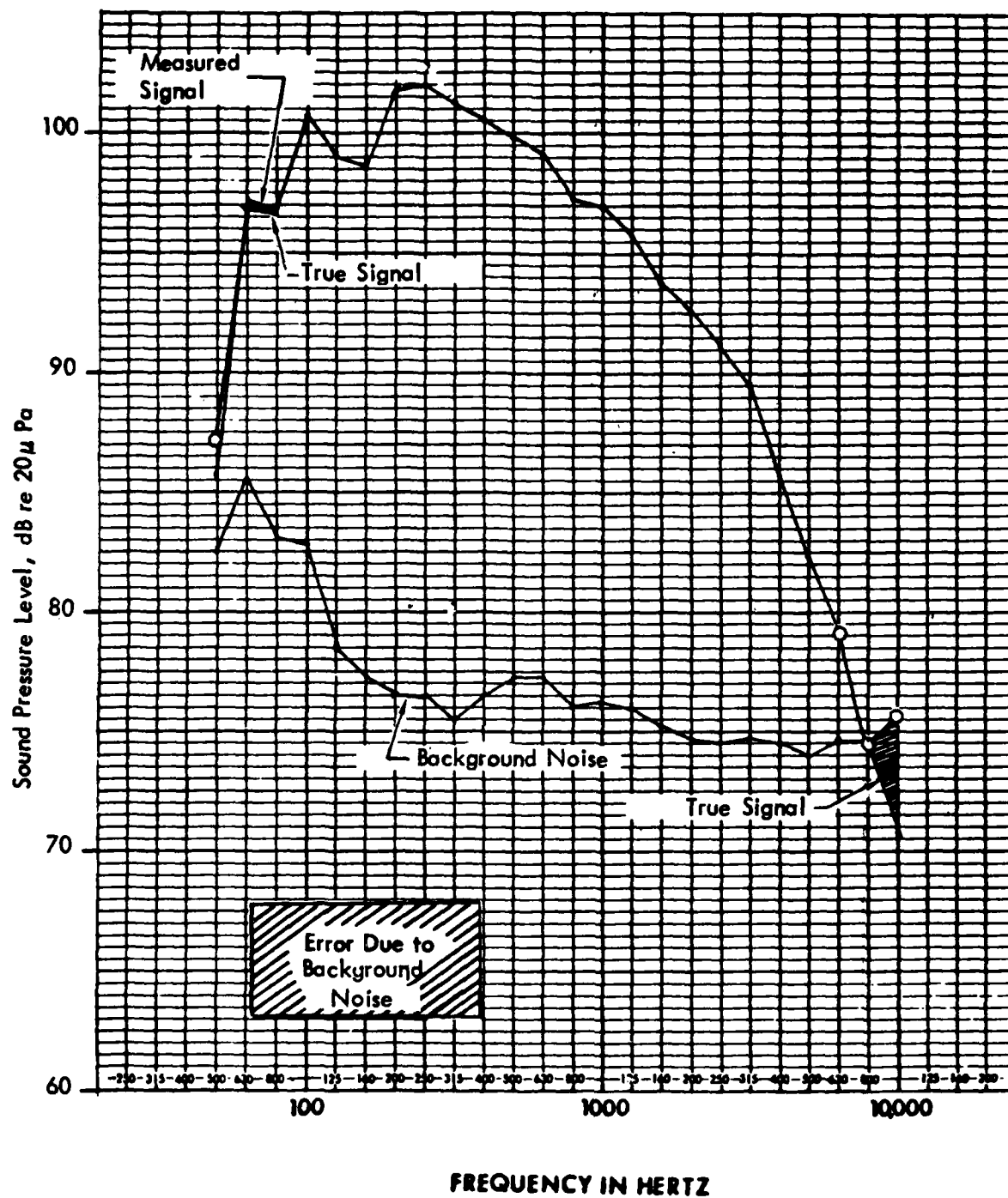
Figure 15. 727 Takeoff with Background Noise Raised to Create Four Bands in Violation of 5 dB Requirement. Bands with o Are Within 5 dB of Background Noise.
