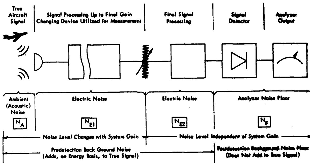
Figure 1. Conceptual Illustration of Elements of Background Noise Encountered in the Acoustic Measurement of Aircraft Noise. The Four Elements Illustrated Can Be Categorized in Two Ways: The First Depends Upon the Way the Background Noise Level Changes with System Gain; the Second Depends Upon the Way the Background Noise Adds, or Does Not Add, to the True Aircraft Noise Signal.
