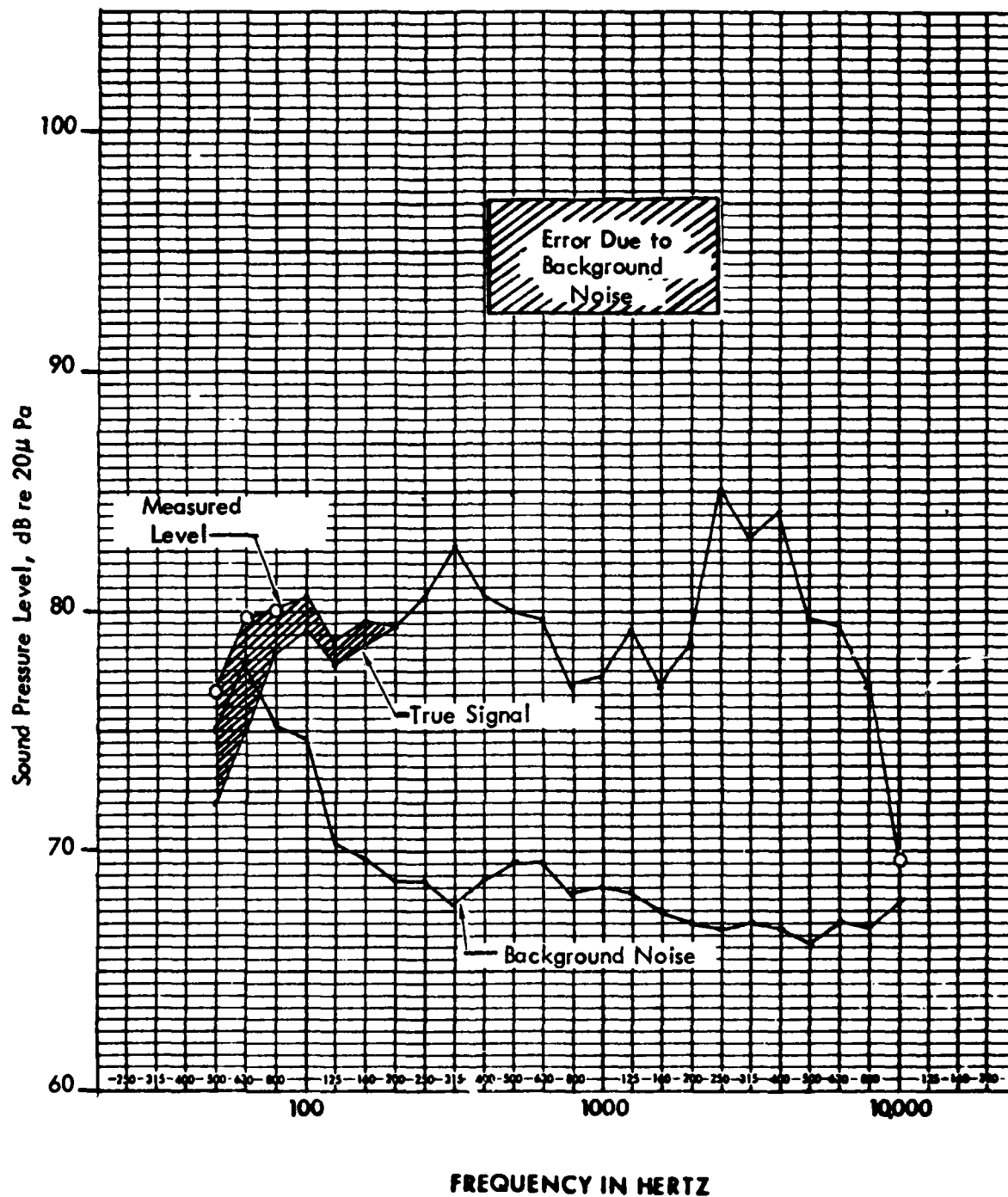
Figure 17. 727 Approach with Background Noise Raised to Create Four Bands in Violation of 5 dB Requirement. Bands with o are Within 5 dB of Background Noise.
