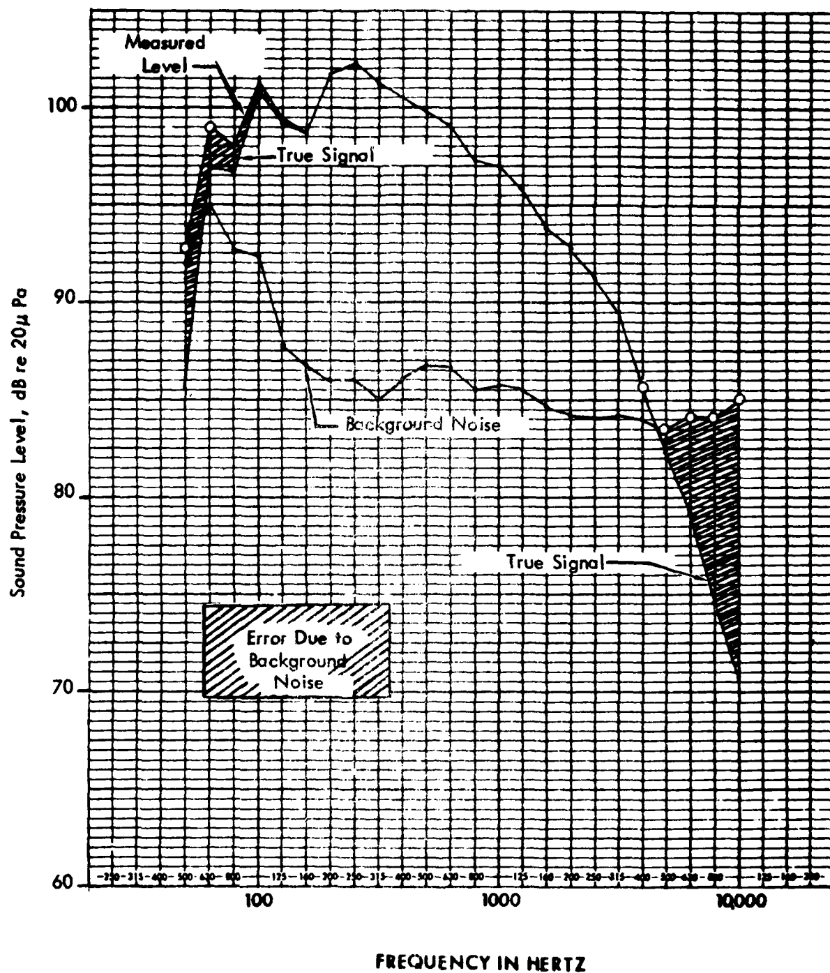
Figure 16. 727 Takeoff with Background Noise Raised to Create Seven Bands in Violation of 5 dB Requirement. Bands with o are Within 5 dB of Background Noise.
