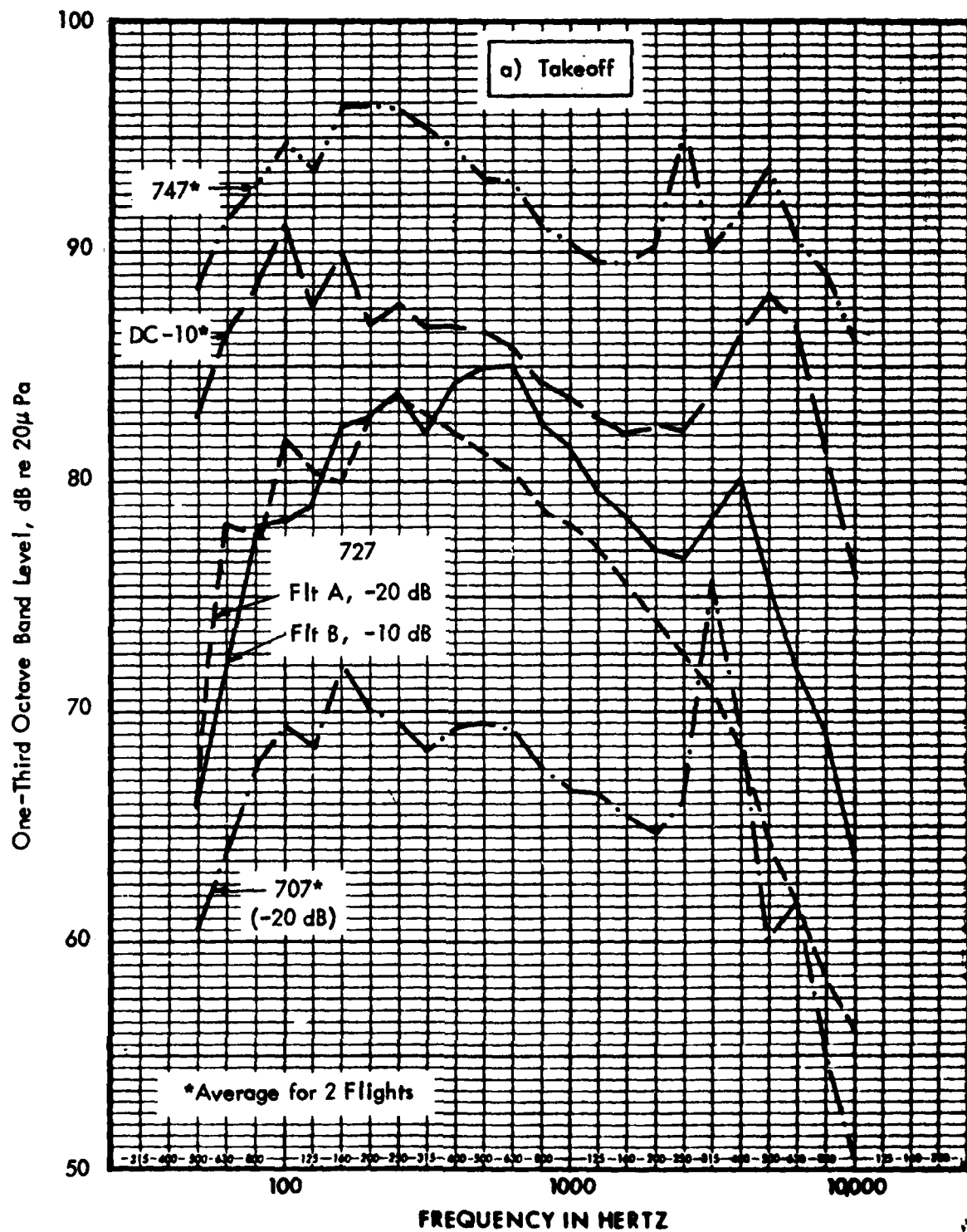
Figure 9. PNLTM Spectra Normalized to 300 m, 25°C, 70% RH - 10 m Microphone over Hard Ground (Some Spectra Displaced Vertically by 10 or 20 dB, as Noted)
