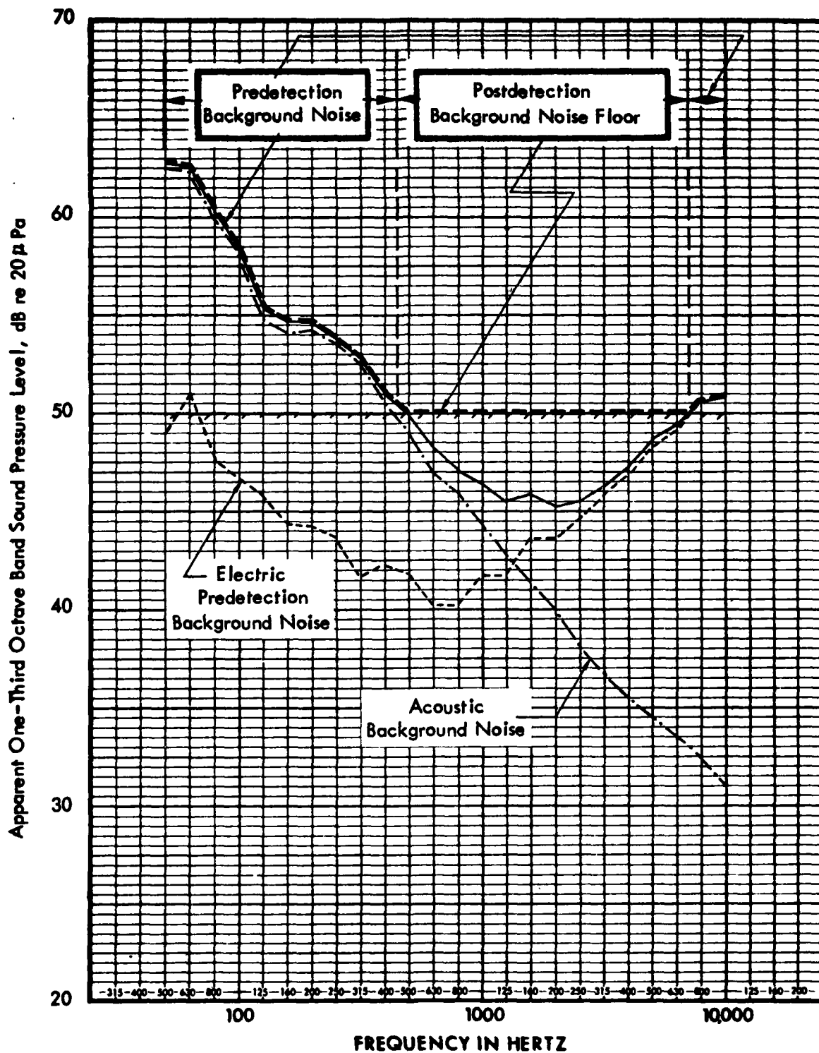
Figure 6. Typical Components of Background Noise in Output of Aircraft Noise Measurement System. This Illustrates a Case Where the Predetection Background Noise Appears at Both the Low and High Frequency End of the Spectrum.
