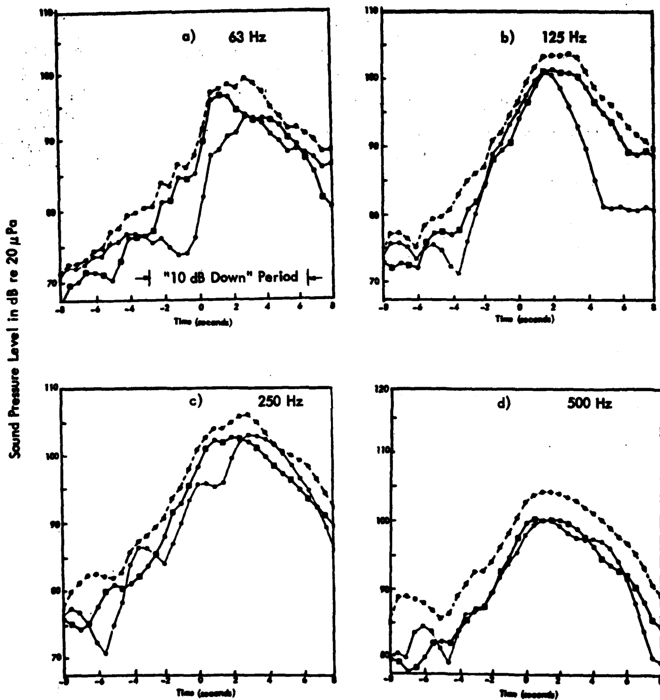
Figure C-1. Time Histories of Selected One-Third Octave Band Levels for 727 at Takeoff - Measured Simultaneously with Three Microphone Positions; —●— for 0.0127 m, —○— for 1.2 m, and —■— for 10 m.
