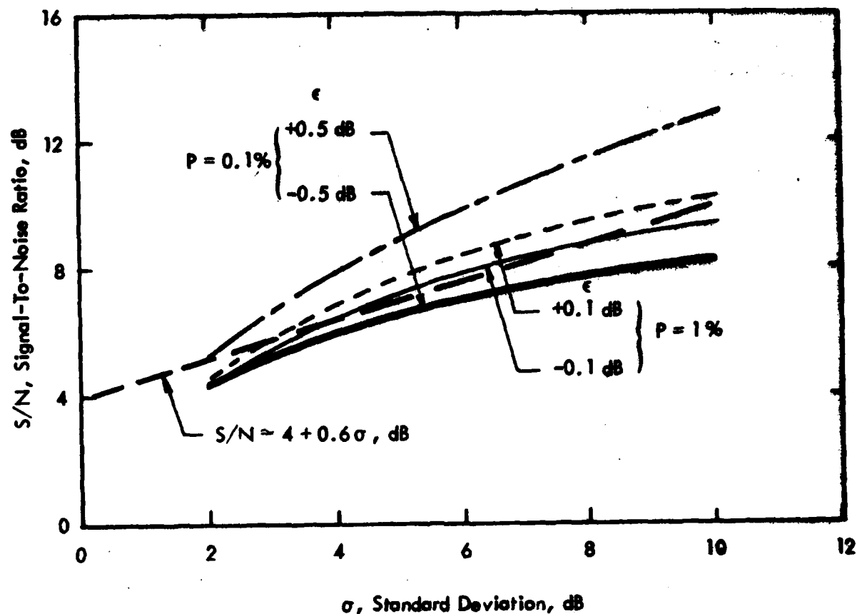
Figure B-4. Required "As Measured" Signal-to-Noise ( S/N ), in dB, as a Function of Standard Deviation ( \sigma ) for Background Noise with Residual Error ( \epsilon ) after Six Separate Tests and Probability ( P ) of Exceeding This Error as Parameters. (Negative Value of Residual Error \epsilon Implies Underestimate of True Aircraft Noise Level.)
