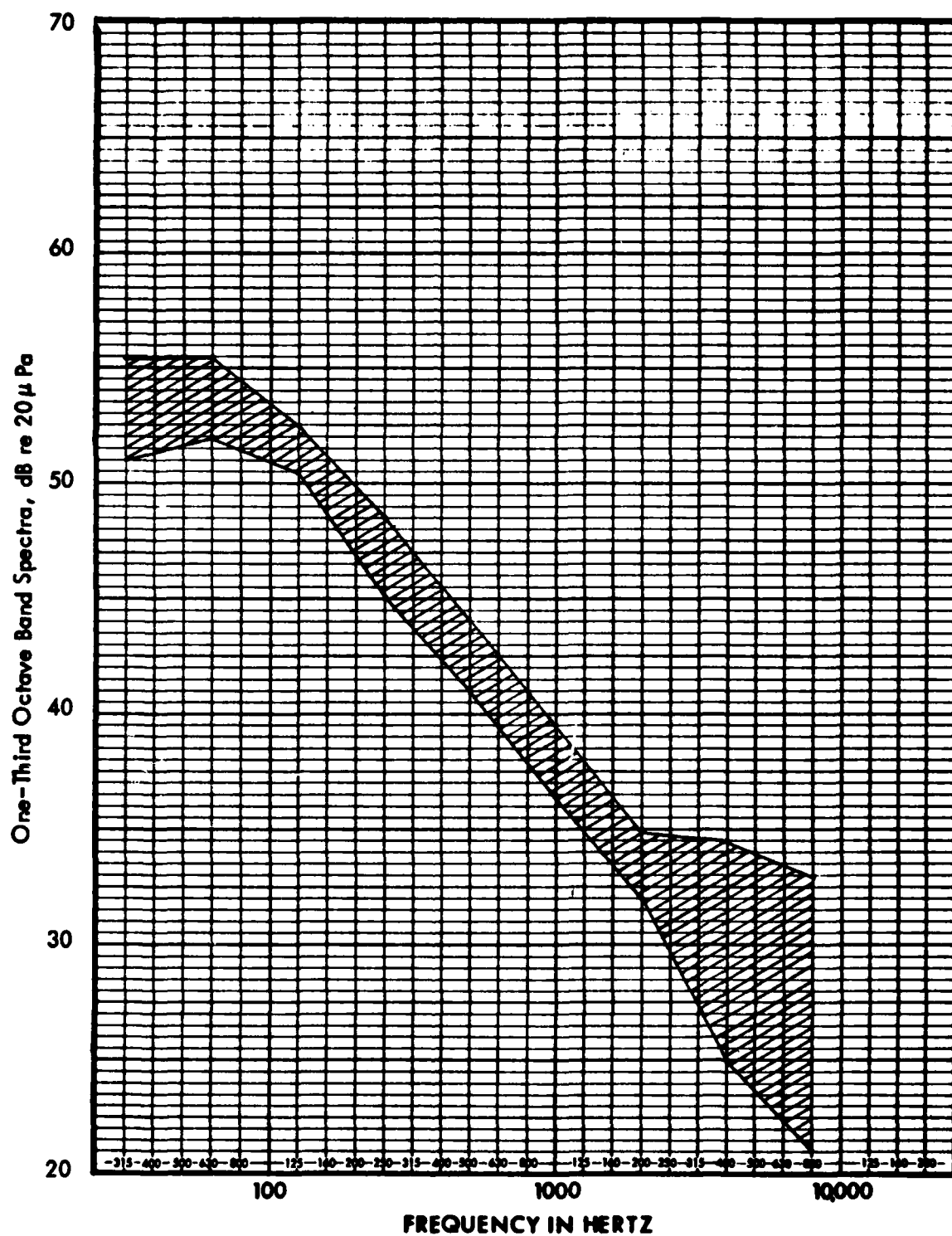
Figure 5. Range of Median One-Third Octave Band Levels of Typical Daytime Ambient Noise in Urban and Suburban Communities; Based on Extensive Octave Band Spectra Measured in Three Different Studies 3, 4, 5
