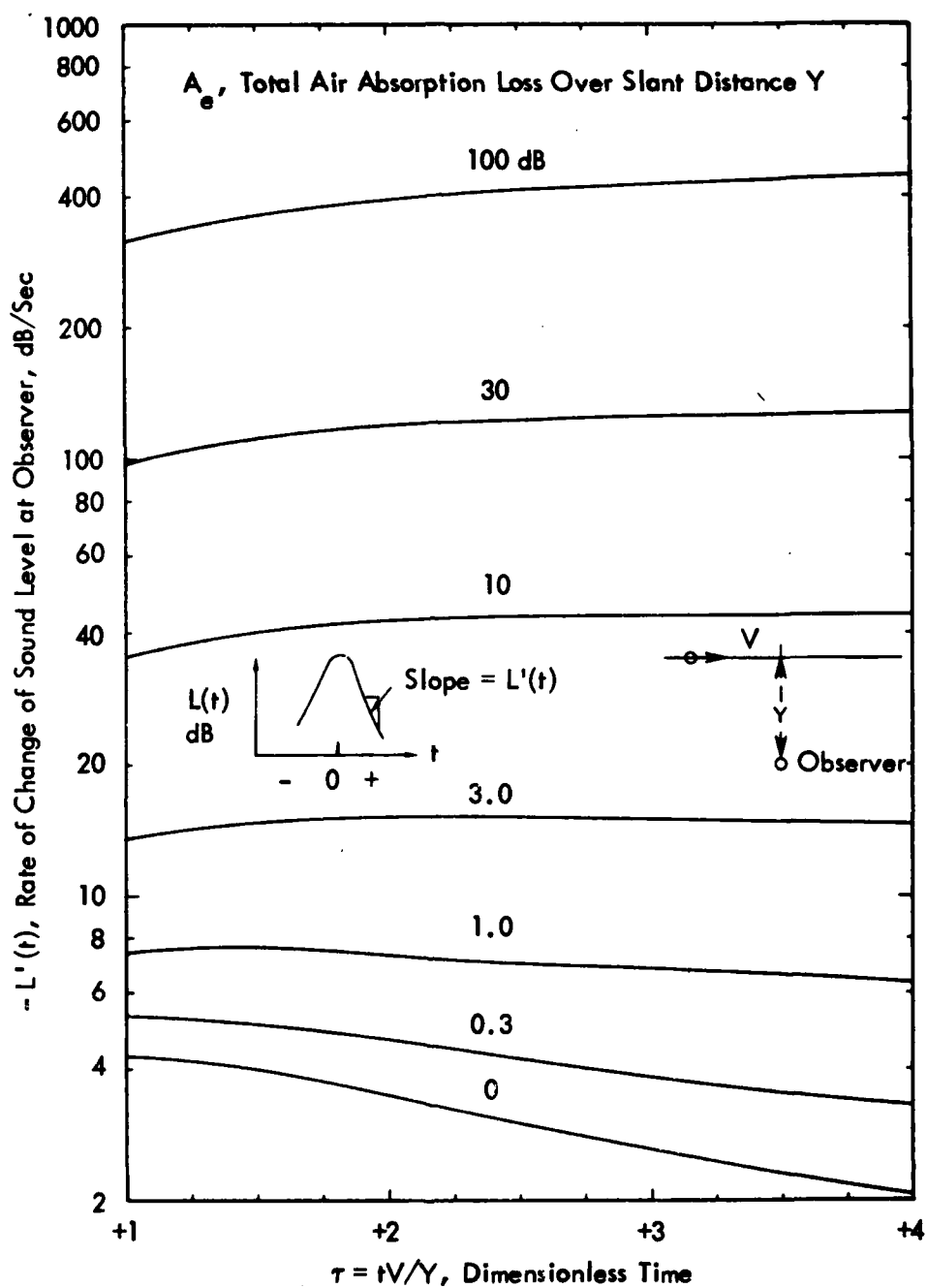
Figure 13. Rate of Change of Level Observed Near Simple Moving Monopole Source in a Uniform, Still, Lossy Atmosphere (See Appendix D for Derivation)
