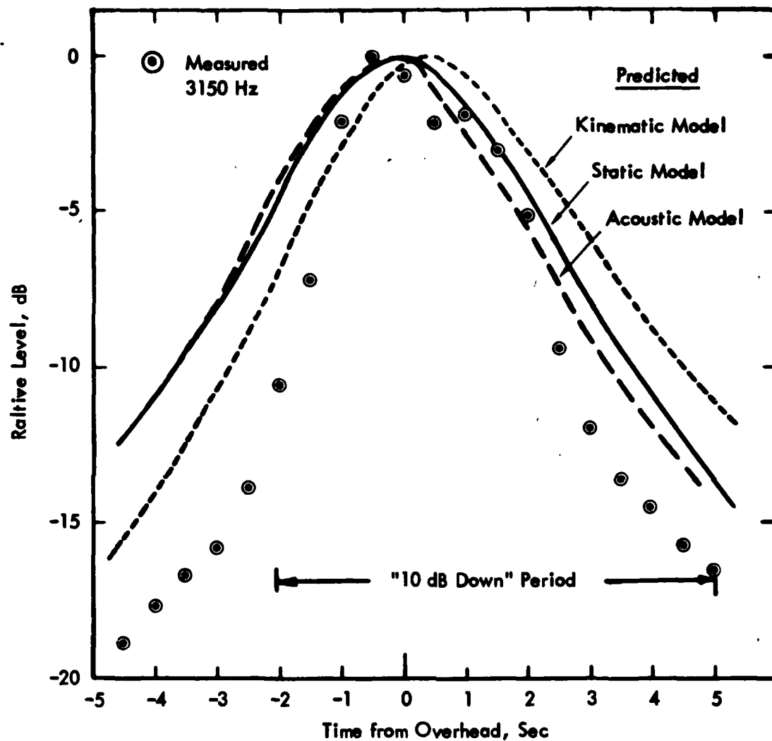
Figure 11. Comparison of Measured Time History of Relative One-Third Octave Band Level at 3150 Hz from 727 on Approach with Values Predicted by Three Different Versions of a Simple Moving Monopole Source Model. (Aircraft Altitude, 127 m, Mach No. = 0.2, Atmospheric Attenuation Coefficient = 1.78 dB/100 m)
