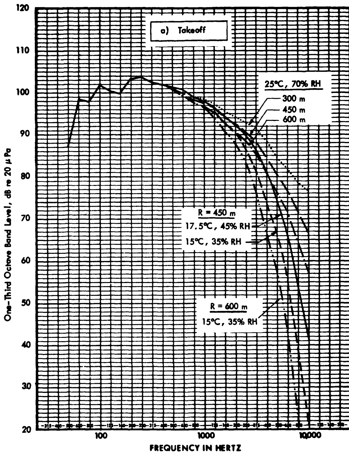
Figure 10. Estimated Variation in PNLTM Spectra for 727 (from Figure 9) Due to Changes in Propagation Distance ( R ) and Weather. (Change in Spreading Loss Not Included)
