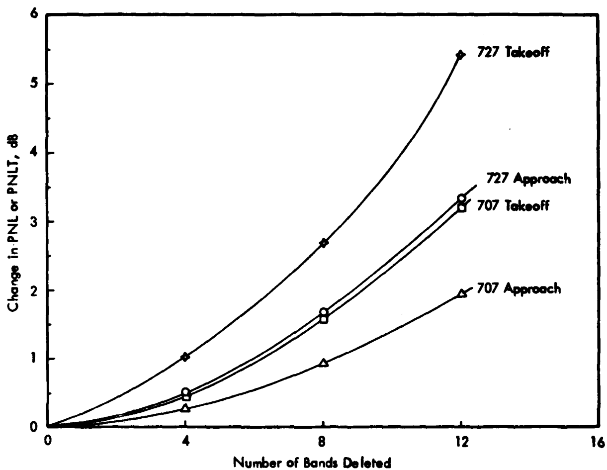
Figure 8. Effect on PNL or PNLT of Deleting Bands for Aircraft Spectra in Figure 7
