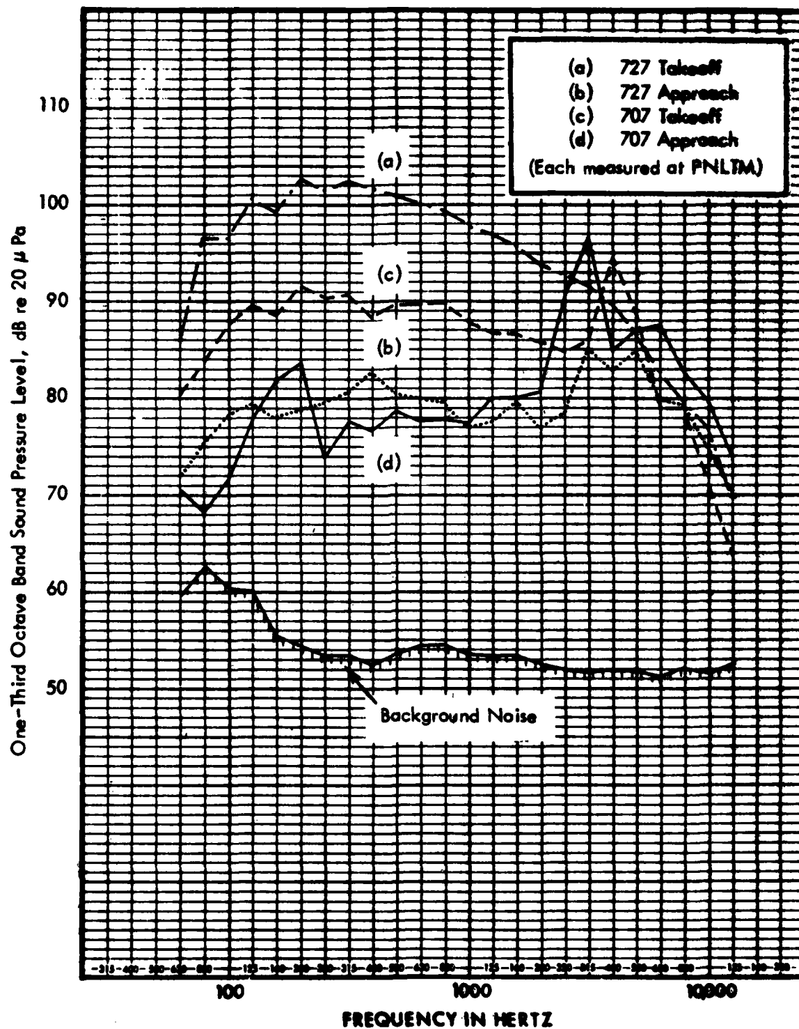
Figure 7. Representative Spectra Used to Demonstrate Effect of Deleting Bands Nearest to Background Noise Spectrum for Computation of PNL
