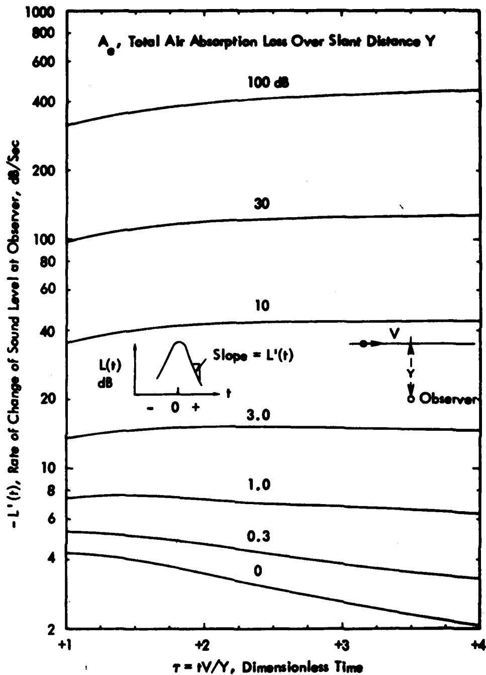
Figure D-1. Rate of Change of Level Observed Near Simple Moving Monopole Source in a Uniform, Still, Lossy Atmosphere
