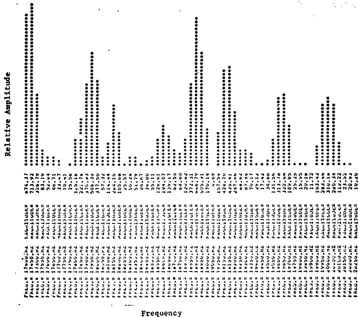
Figure 27g. Power spectral Density for Y/D = 0, X/D = 3, 17400 - 20250 Hz.
