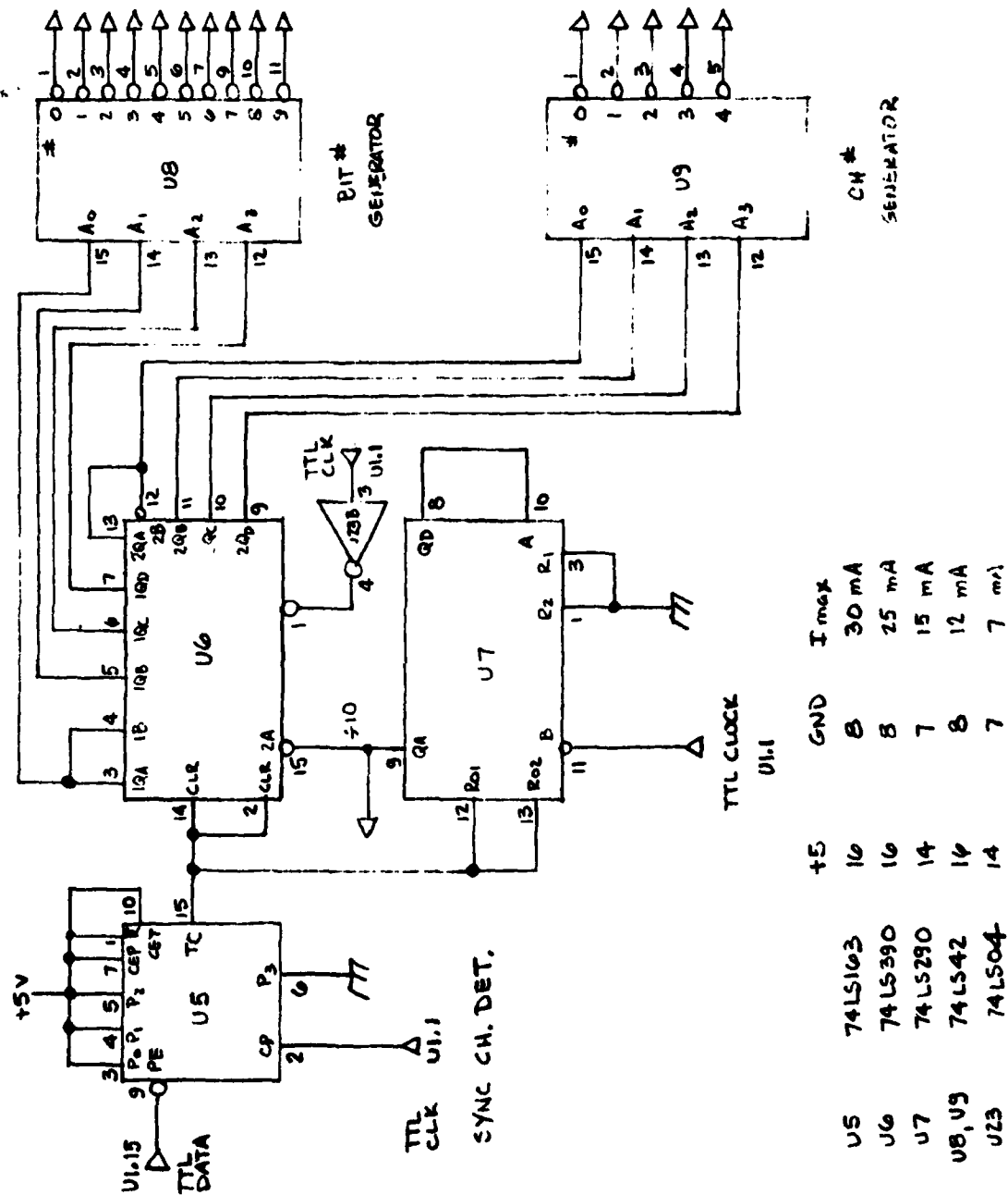
FIGURE 15 TIMING GENERATOR
