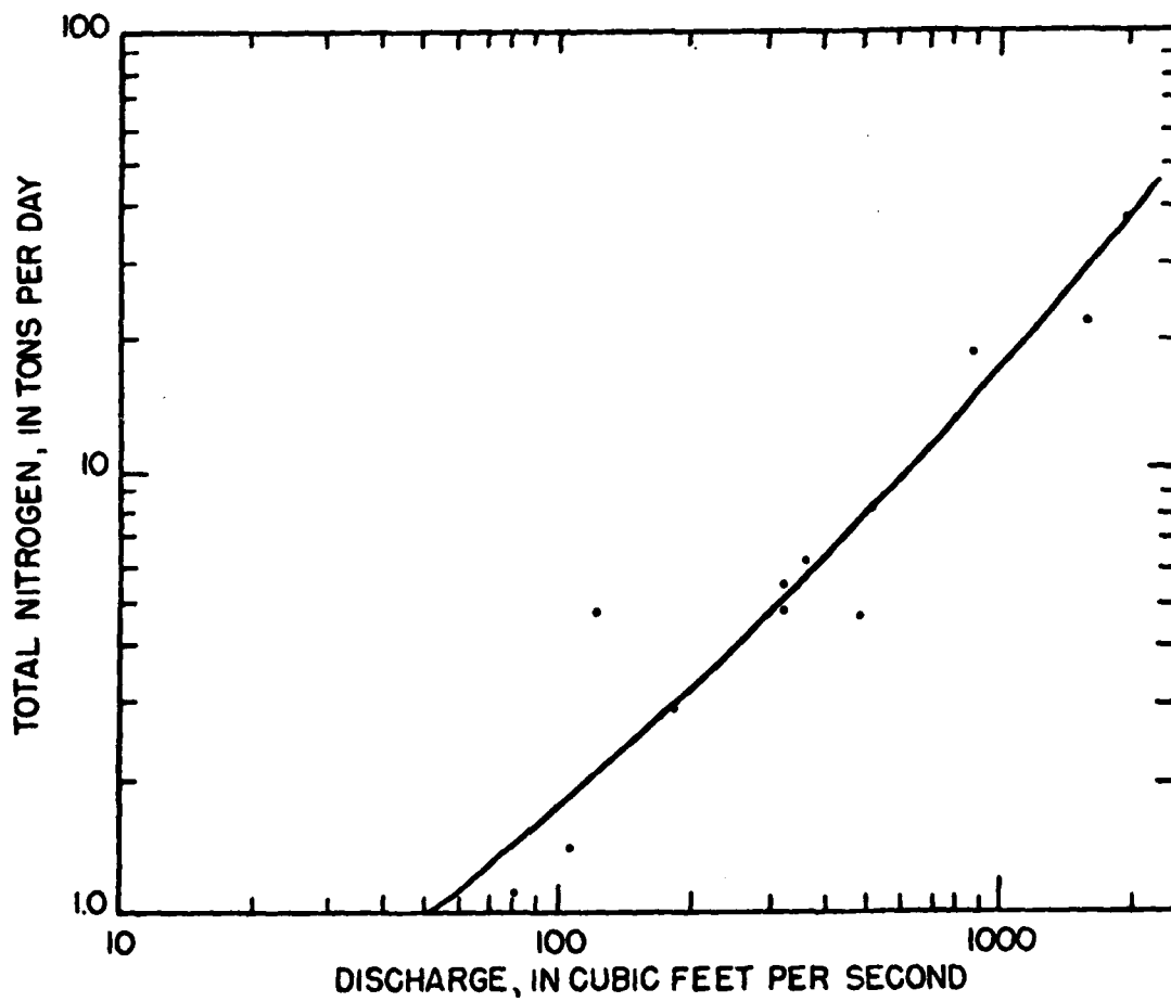
Figure 3.--Graph showing relation between discharge and total nitrogen in Tulpehocken Creek basin near Blue Marsh Dam site.
