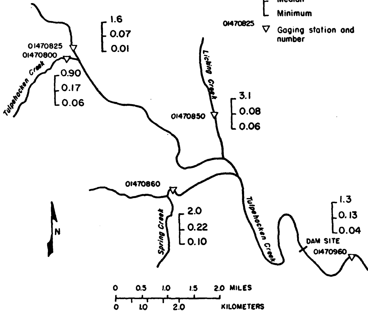
Figure 2.--Map showing total phosphorus concentrations in Tulpehocken Creek basin.
