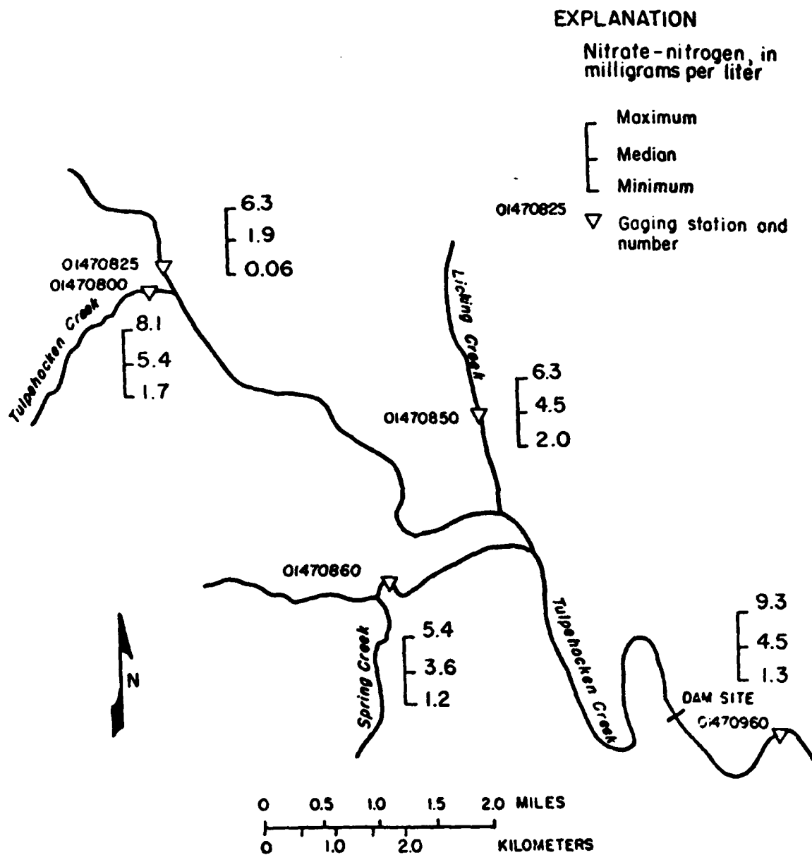
Figure 1.--Map showing nitrate-nitrogen concentrations in the Tulpehocken Creek basin.
