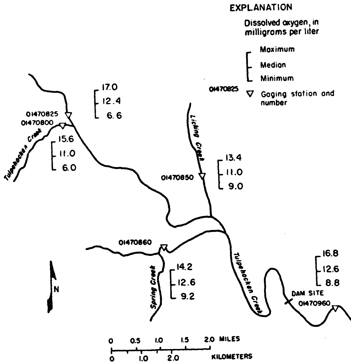
Figure 4.--Map showing dissolved oxygen concentrations in the Tulpehocken Creek basin.
