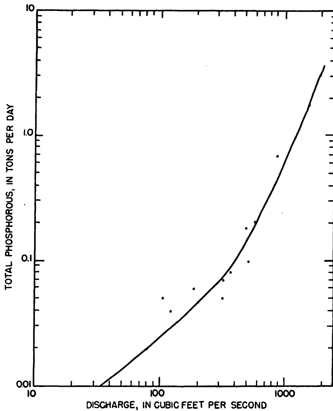
Figure 5'.--Graph showing relation between discharge and total phosphorus in Tulpehocken Creek basin near Blue Marsh Dam site.
