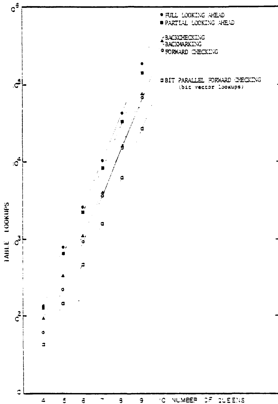
Figure 10 shows the number of table lookups used to find all solutions to the N-queens problem for varying N, with the natural unit order.
