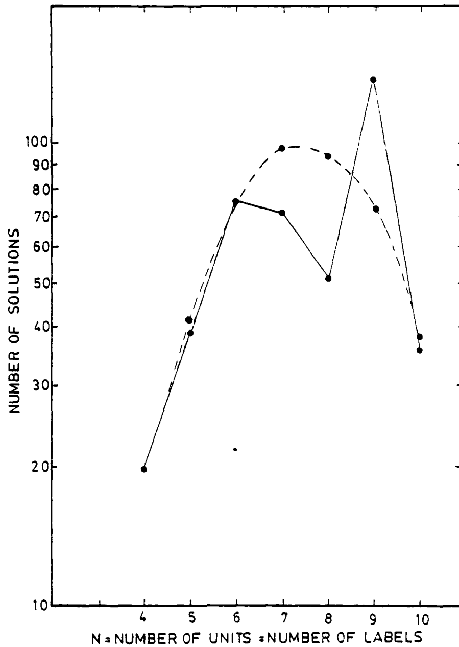
Figure 9 shows the average number of solutions for the probabilistic relations in figure 8. This is the average of 5 experiments for each problem size, and relations are random with consistency check success probability p=0.65 . The dotted curve is the expected number of solutions.
