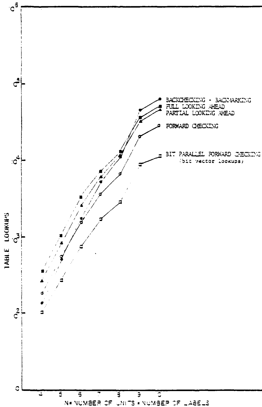
Figure 11 shows the number of table lookups for the average of 5 random relations at each N, with number of units = number of labels = N, and probability of consistency check success p = 0.65 . These random problems are the same as shown in figures 8 and 9.
