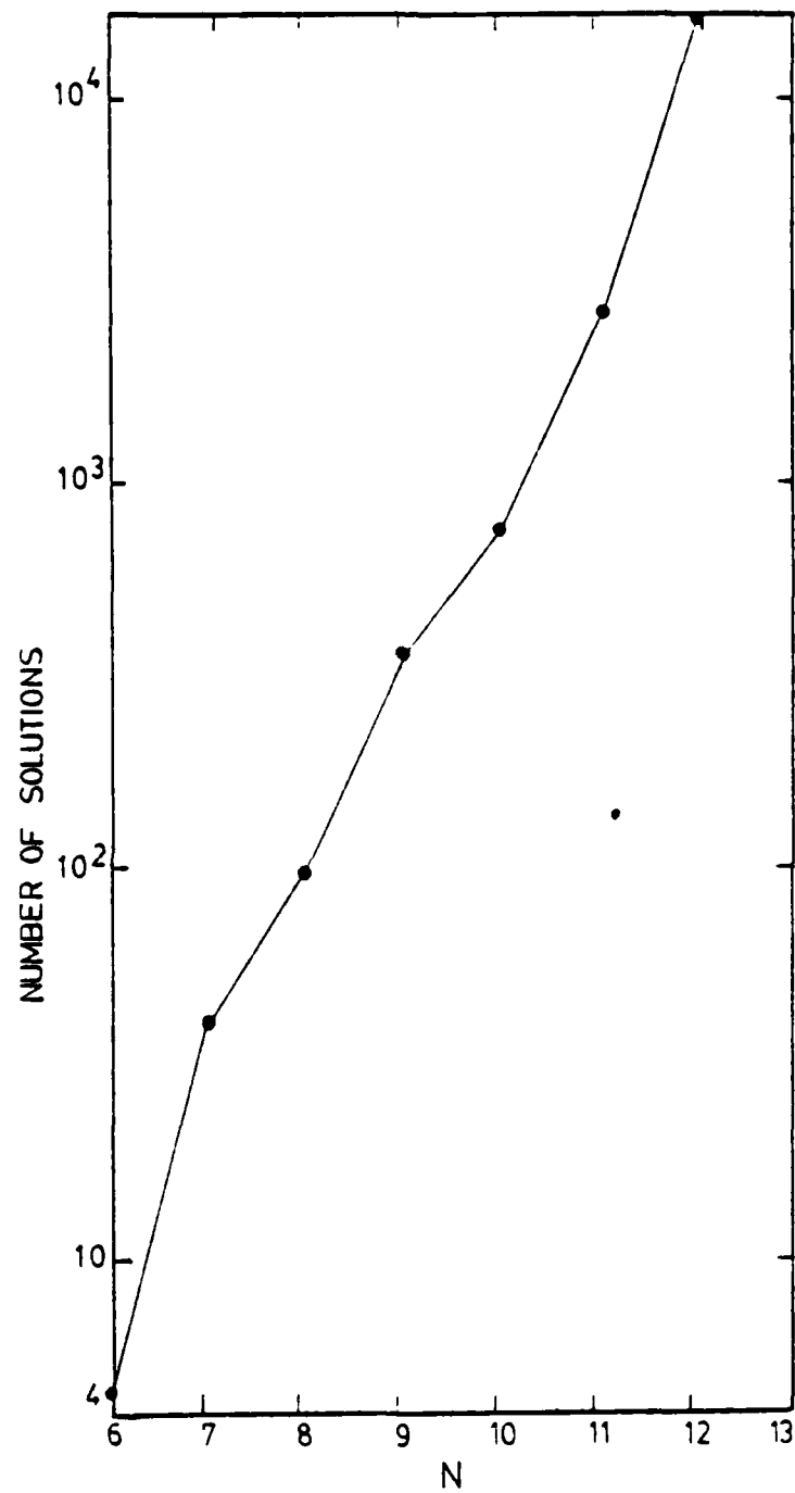
Figure 7 illustrates the number of solutions for the N-queens problem.
