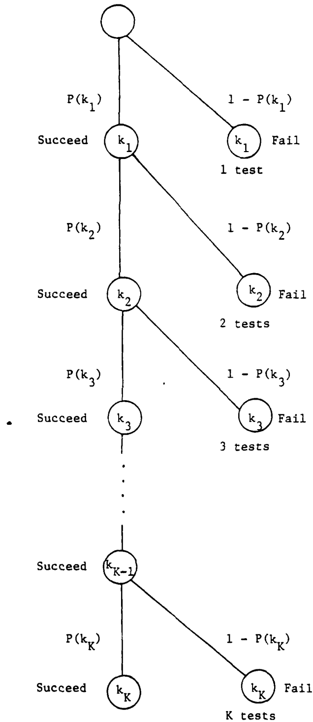
Figure 34 illustrates the K+1 outcomes of K tests.
