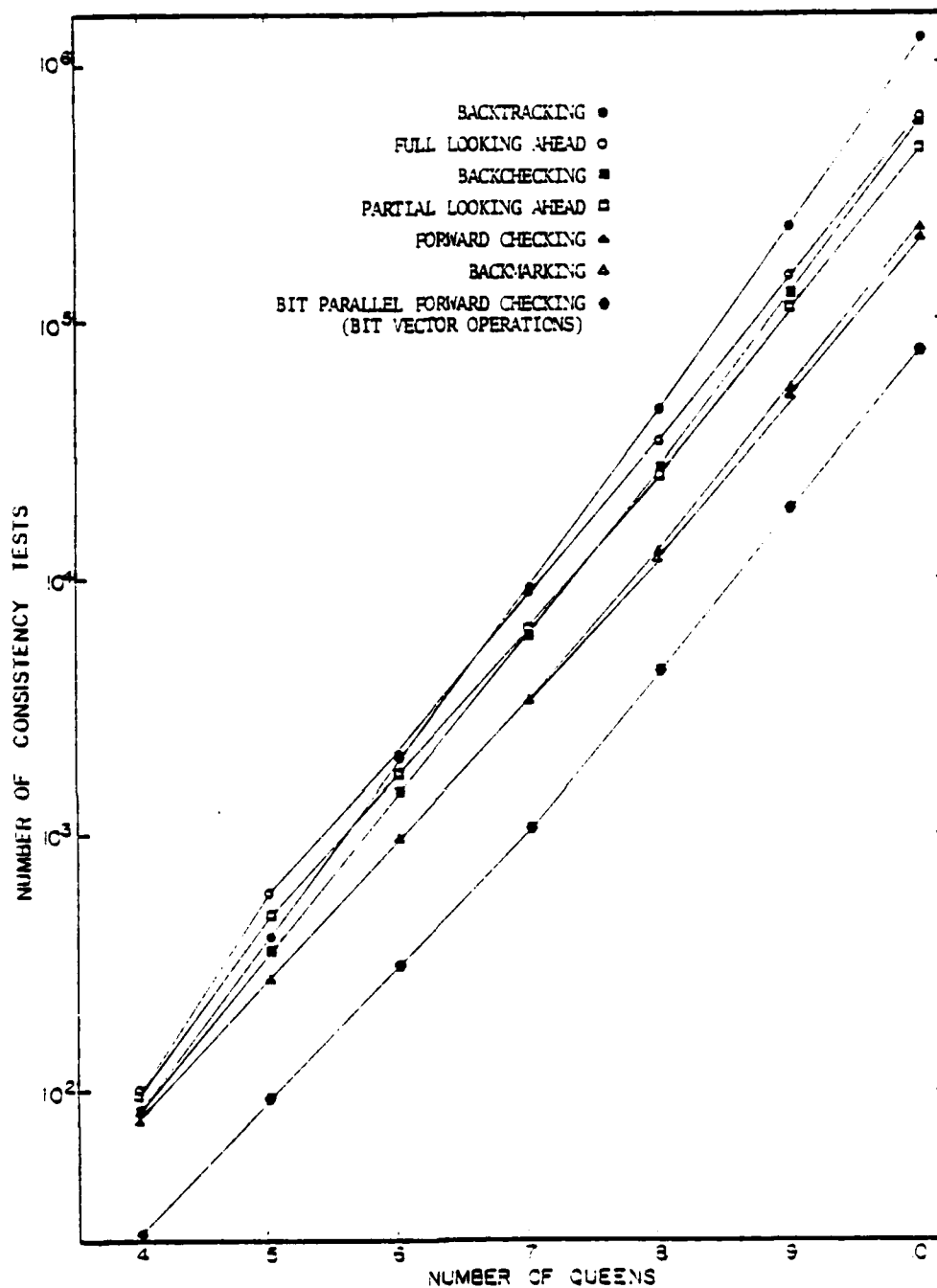
Figure 6 compares the efficiency of the standard backtracking procedure with backchecking, looking ahead, forward checking, and backmarking, for the N-queens problem in the natural unit order. The number of bit vector operations for bit parallel forward checking is also shown.
