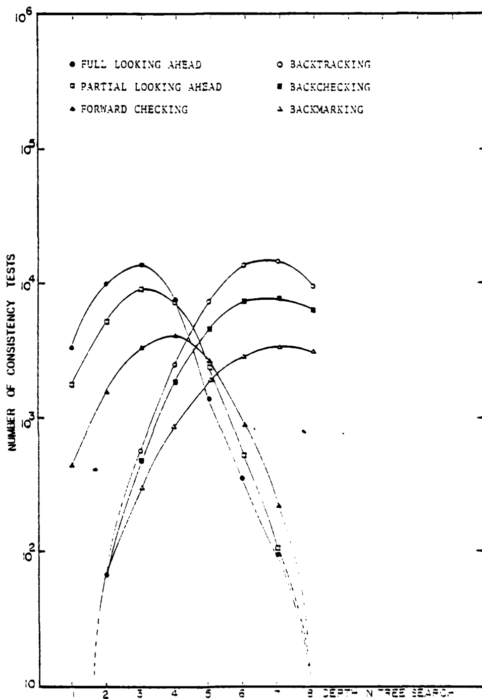
Figure 19 compares the number of consistency tests made at each level in the tree search for six different procedures, for the 8-queens problem, in the natural unit order.
