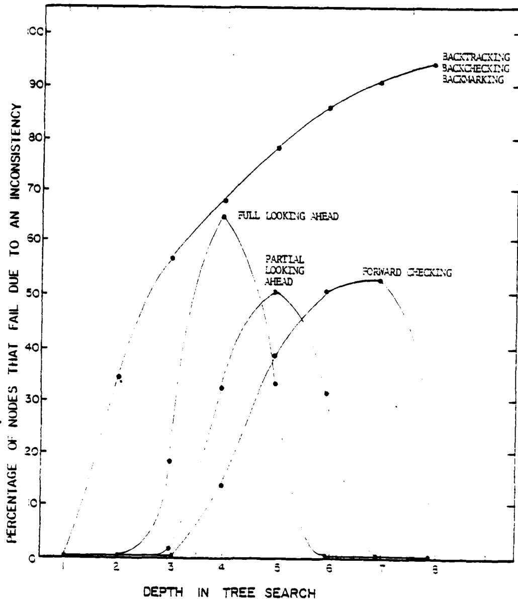
Figure 21 shows the percentage of nodes at a given depth in the tree search which fail because some inconsistency is detected at that node. Results are shown for the various algorithms in the 8-queens problem. Backchecking and backmarking often discover that there is an inconsistency by using table lookups, rather than performing all the checks. Nodes in the lookahead type algorithms fail because a future unit fails to have any remaining labels after inconsistent future labels are removed.
