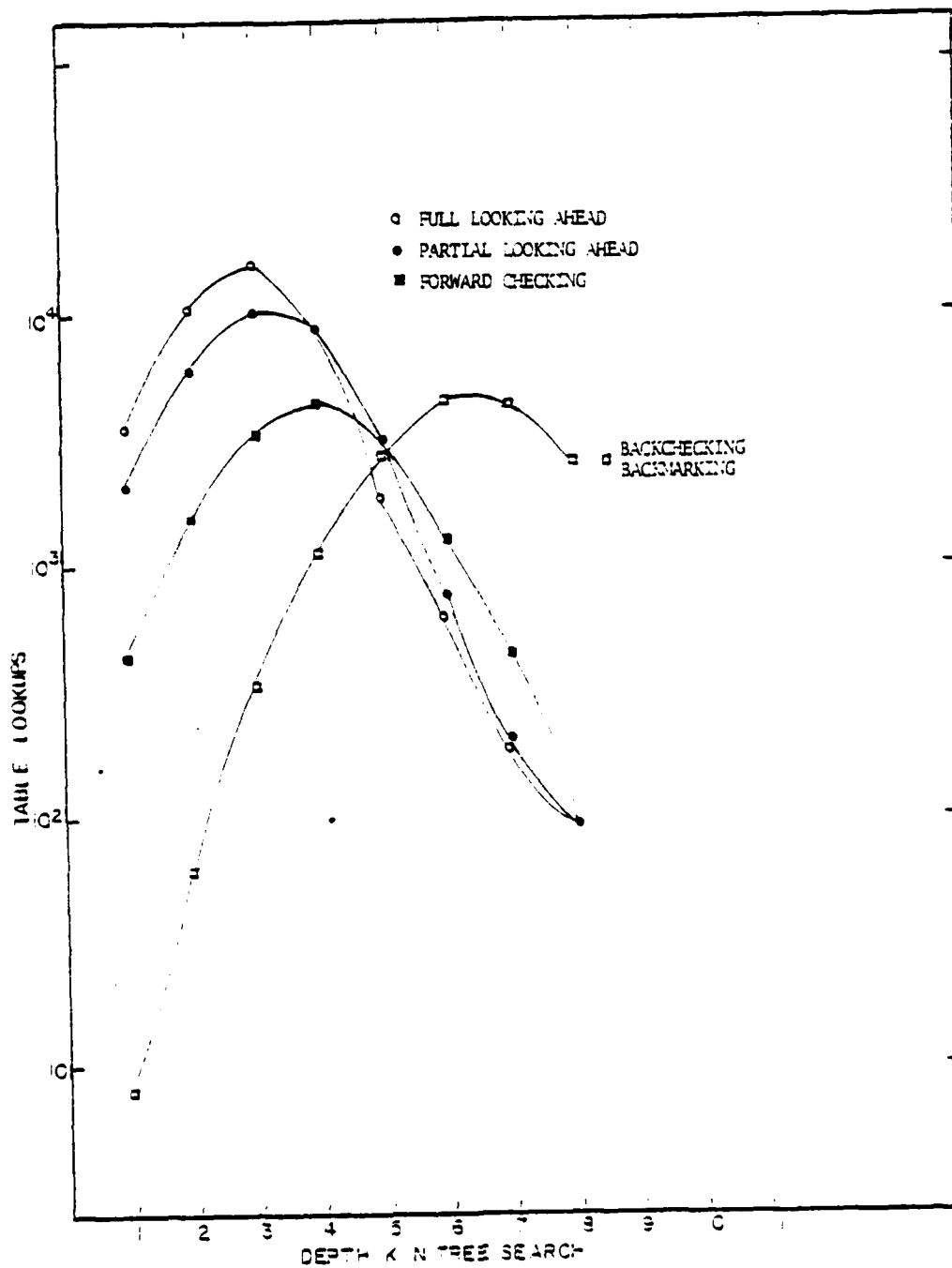
Figure 20 shows the number of table lookups at each possible depth k in the tree search to find all solutions to the 8-queens problem, for the various algorithms.
