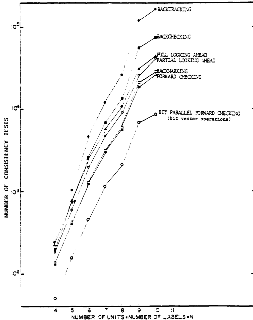
Figure 8 represents the number of consistency tests in the average of 5 runs of the indicated programs. Relations are random with consistency check probability p=0.65 and number of units = number of labels = N . Each random relation is tested on all 6 methods, using the same 5 different relations generated for each N . The number of bit-vector operations in bit parallel forward checking is also shown for the same relations.
