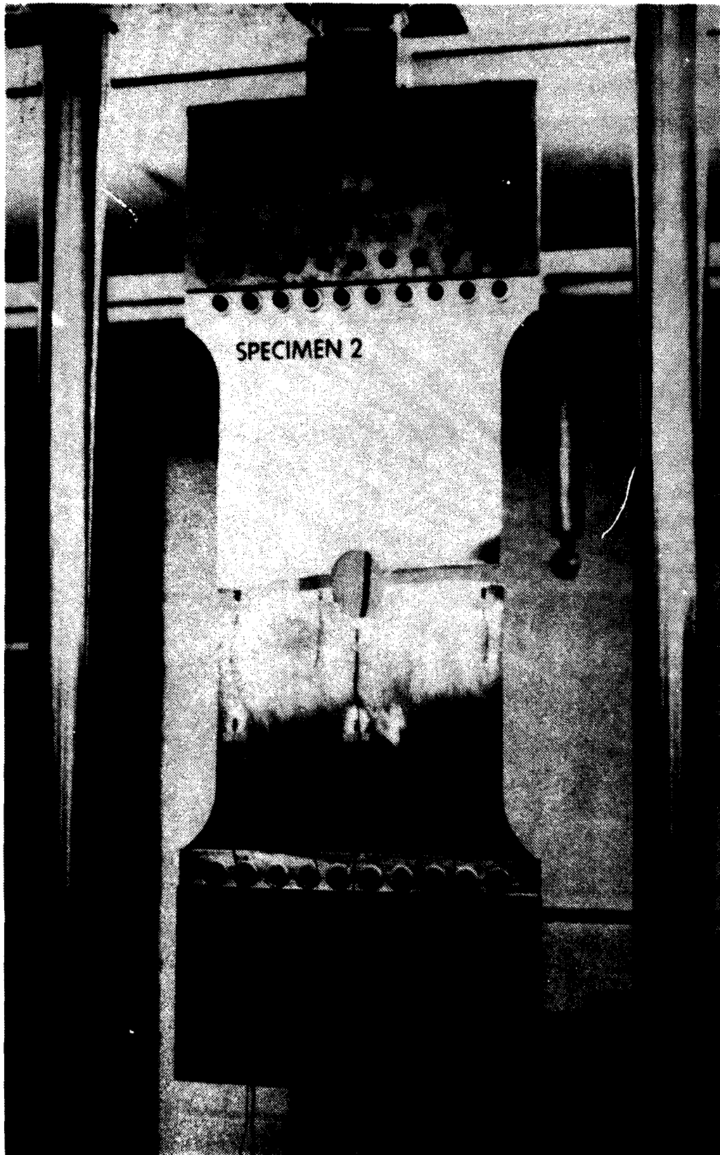
PHOTOGRAPH 5 PANEL SPECIMEN WITH HOLE PENETRATION PREPARATION AFTER TEST
