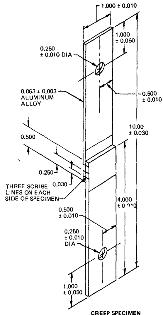
CREEP SPECIMEN
