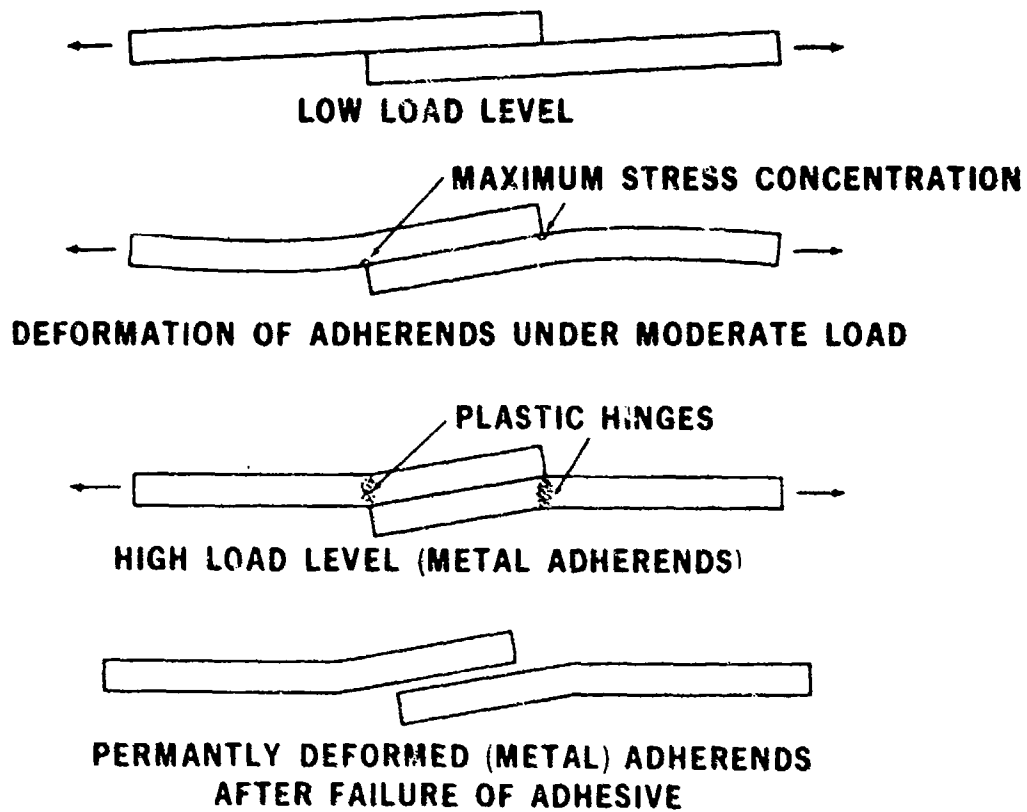
FIGURE 43. FAILURE OF SINGLE-LAP BONDED JOINTS WITH YIELDING ADHERENDS
