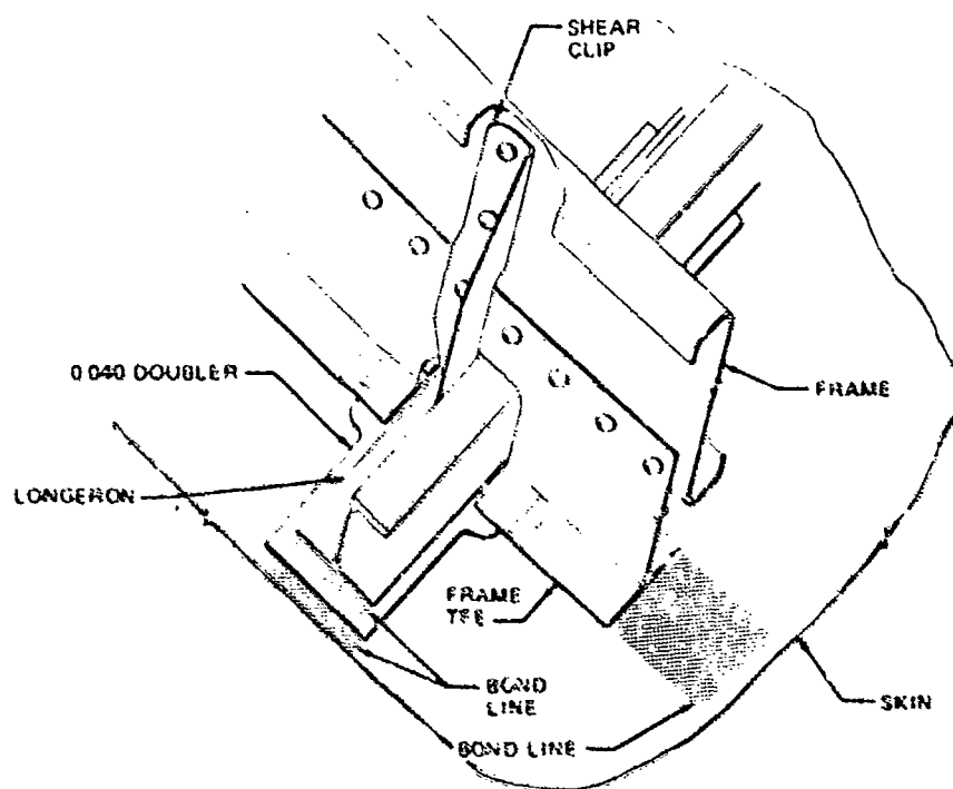
FIGURE 70 . TYPICAL FRAME AND INTERNAL LONGERON INTERSECTION WITH DOUBLER TO PROVIDE STRUCTURAL CONTINUITY
