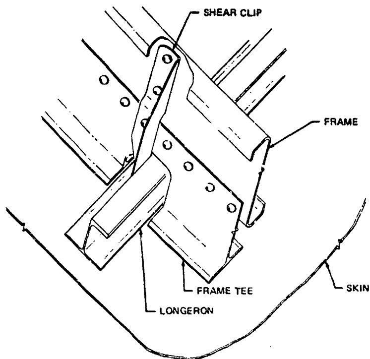
FIGURE 69 . POORLY-DETAILED TYPICAL FRAME AND INTERNAL LONGERON INTERSECTION (DISCONTINUITY IN FRAME TEE)
