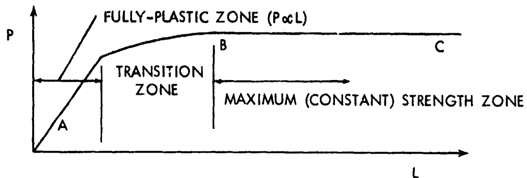
EFFECT OF LAP LENGTH ON ADHESIVE-BONDED JOINT STRENGTH
