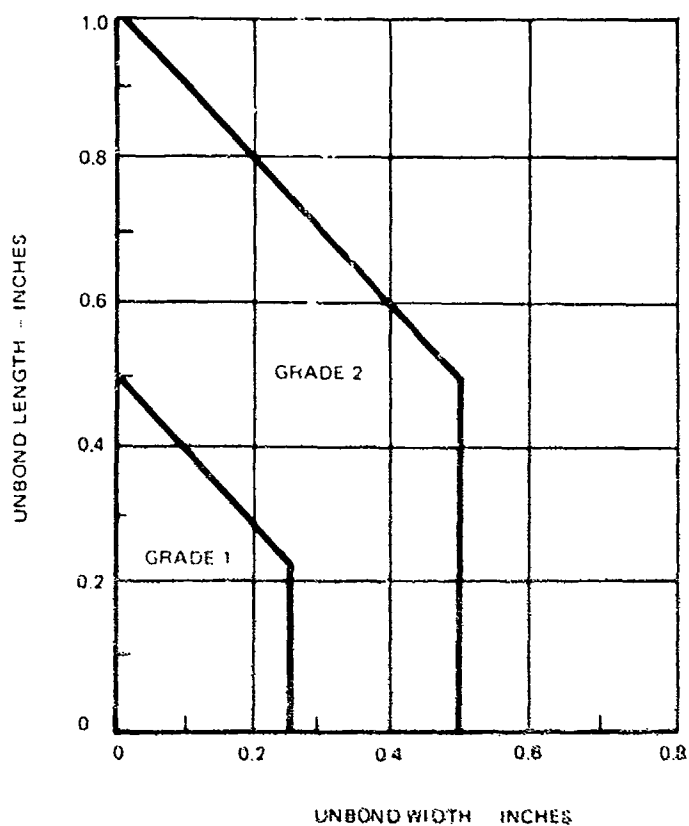
FIGURE 16 CRITICAL AREA OF BONDLINE
