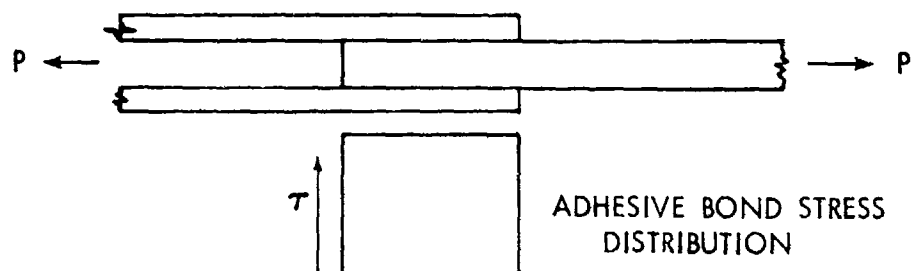
EFFECT OF LAP LENGTH ON ADHESIVE-BONDED JOINT STRENGTH
