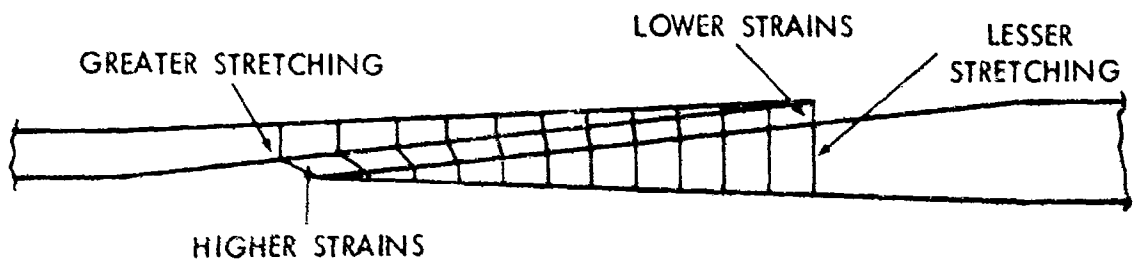
(C) NON-UNIFORM ADHESIVE DEFORMATION BECAUSE OF DISSIMILAR STRETCHING OF DIFFERENT ADHERENDS
