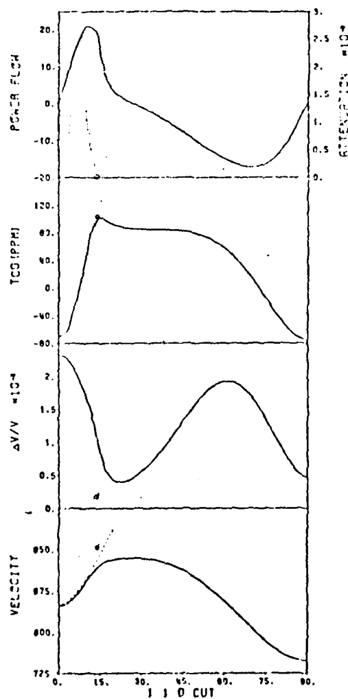
FIG. 13. SAW and Pseudo SAW Properties of \text{Ti}_3\text{TaSe}_4 for \langle 110 \rangle cut.
