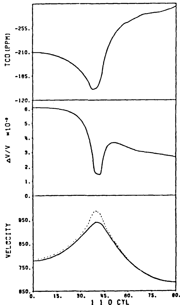
FIG. 16. SAW and Bulk Wave Properties of Tl_3TaS_4 for \langle 110 \rangle Axis cylinder Cut. Solid Curves: SAW Properties. Dashed Curves: Transverse Bulk Velocity.
