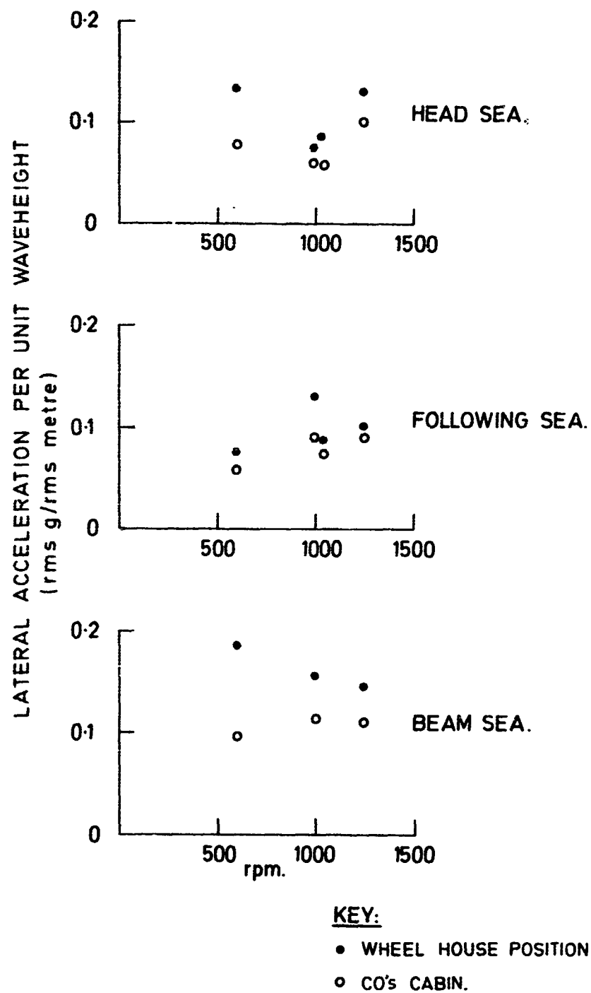
Fig.70. Lateral acceleration per unit waveheight.
