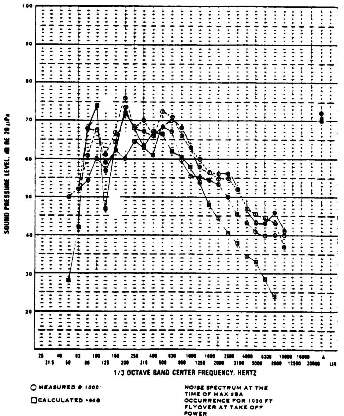
FIGURE 2. PIPER PA28-20 ARROW II FLYOVER NOISE
