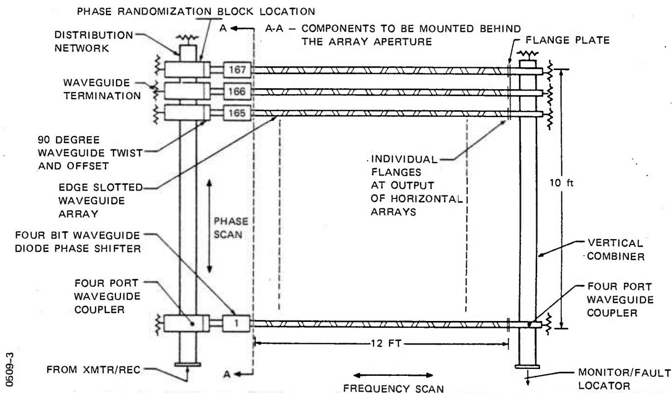
Figure 2-3. Antenna waveguide configuration and signal flow.
