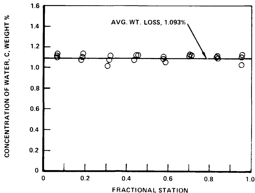
FIGURE 41 MOISTURE DISTRIBUTION IN LAMINATE 2 COUPON 2SF1133-B8 AFTER 127 DAYS OF CONDITIONING AT 82.2°C (180°F) AT 90% R.H. AND EXPOSED 5 MIN. AT 82.2°C (180°F) IN LABORATORY AIR DURING TENSION TEST
