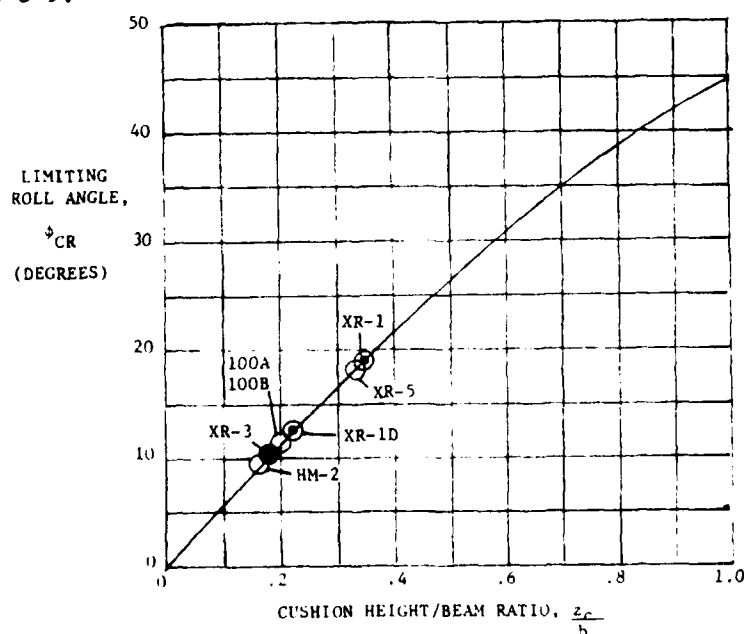
FIGURE 3-9. VARIATION OF LIMITING ROLL ANGLE WITH CUSHION HEIGHT/BEAM RATIO (AT \phi = \phi_{CR} THE WET DECK BEGINS TO BE IMMERSSED).
