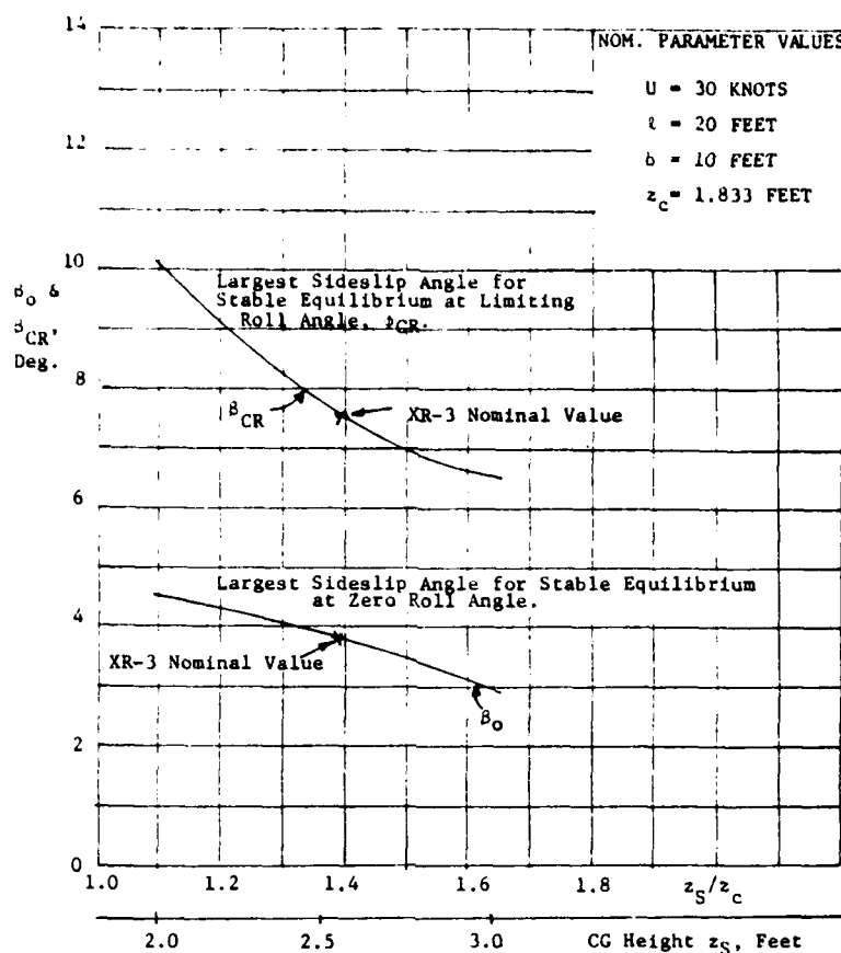
FIGURE 3-16. VARIATION OF SIDESLIP ANGLE WITH C.G. HEIGHT z_S FOR LIMITS OF ROLL STABILITY. (AGC MAY 69)
