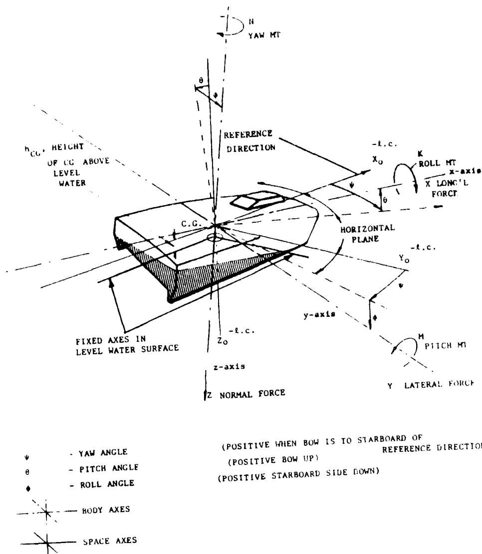
FIGURE 6-4. DEFINITION OF AXIS SYSTEM.
