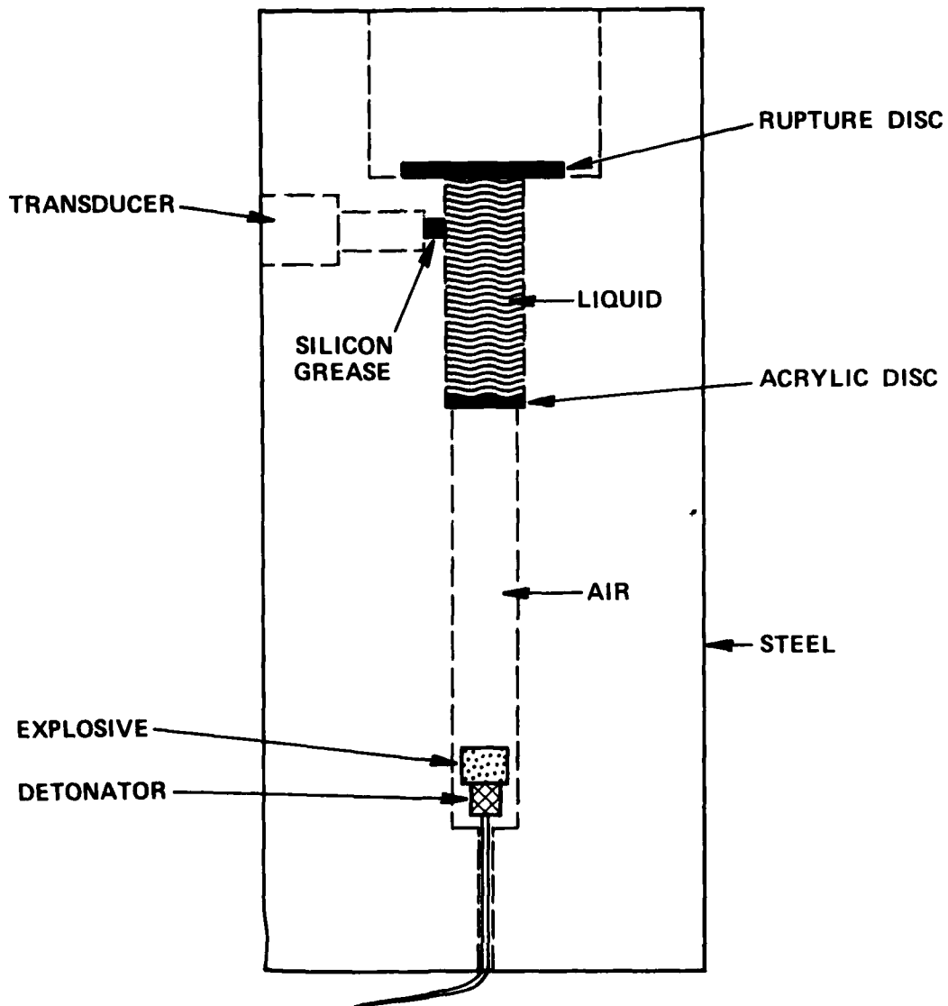
Figure 3. Cross-Sectional View of Explosive Projector
