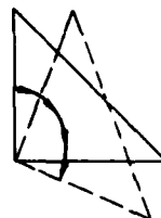
Figure 2.4. Complex Transformations
