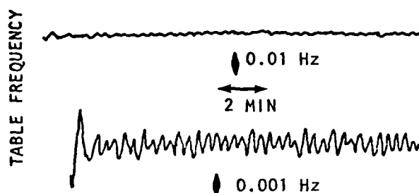
Fig. 33. Effect on table motion of relaxing the neutral position tension of the springs. The beating has decreased, but the first harmonic acceleration has increased.
