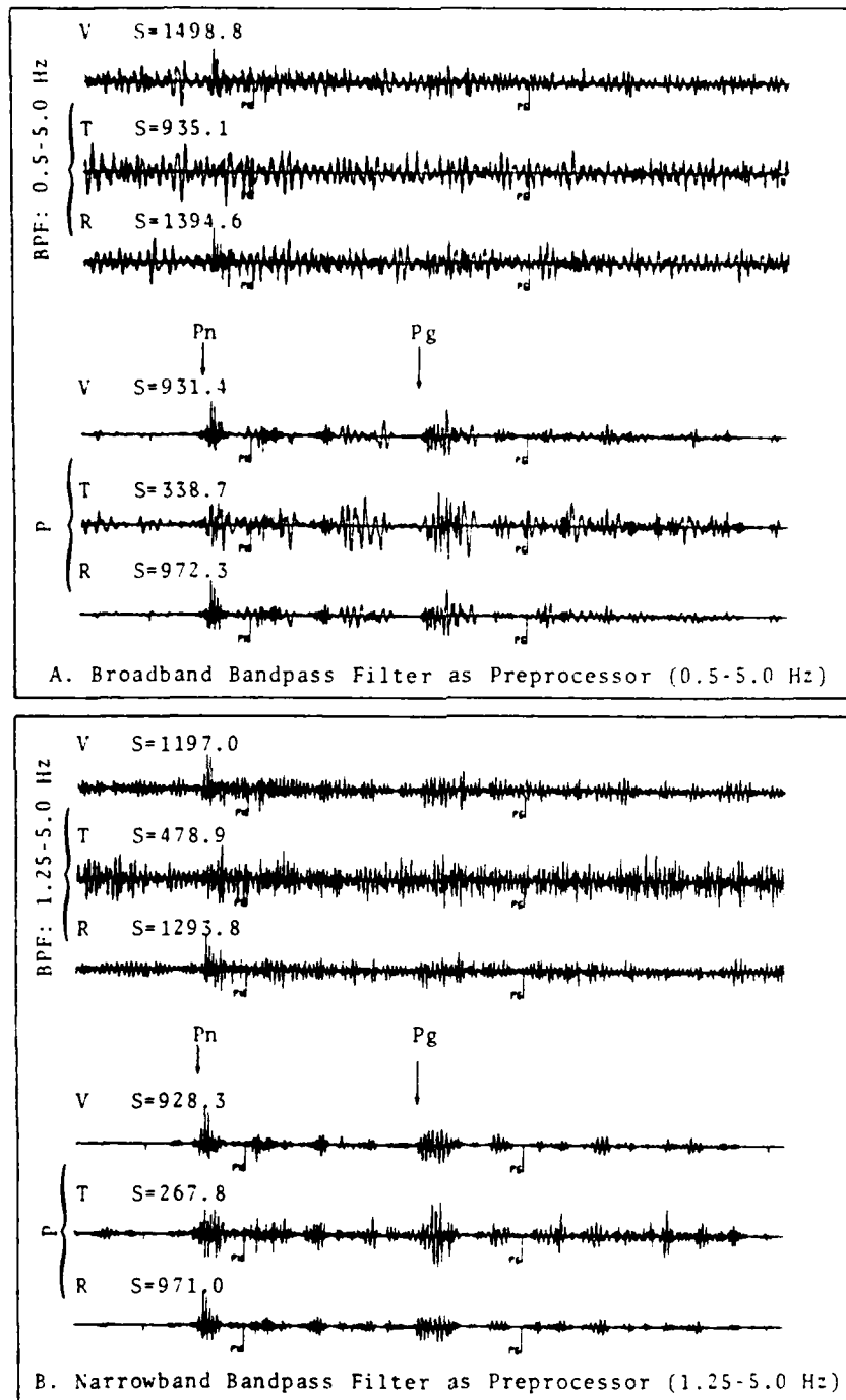
FIGURE IV-1 EXTRACTION OF Pn AND Pg PHASES
