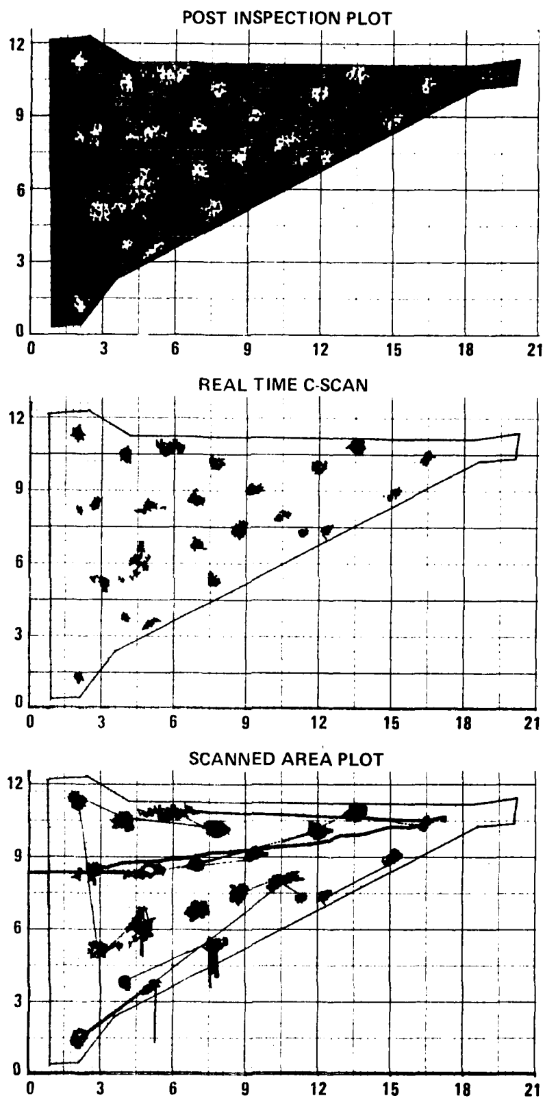
Figure 22 Flaw and Scan Plots for Specimen A-3
