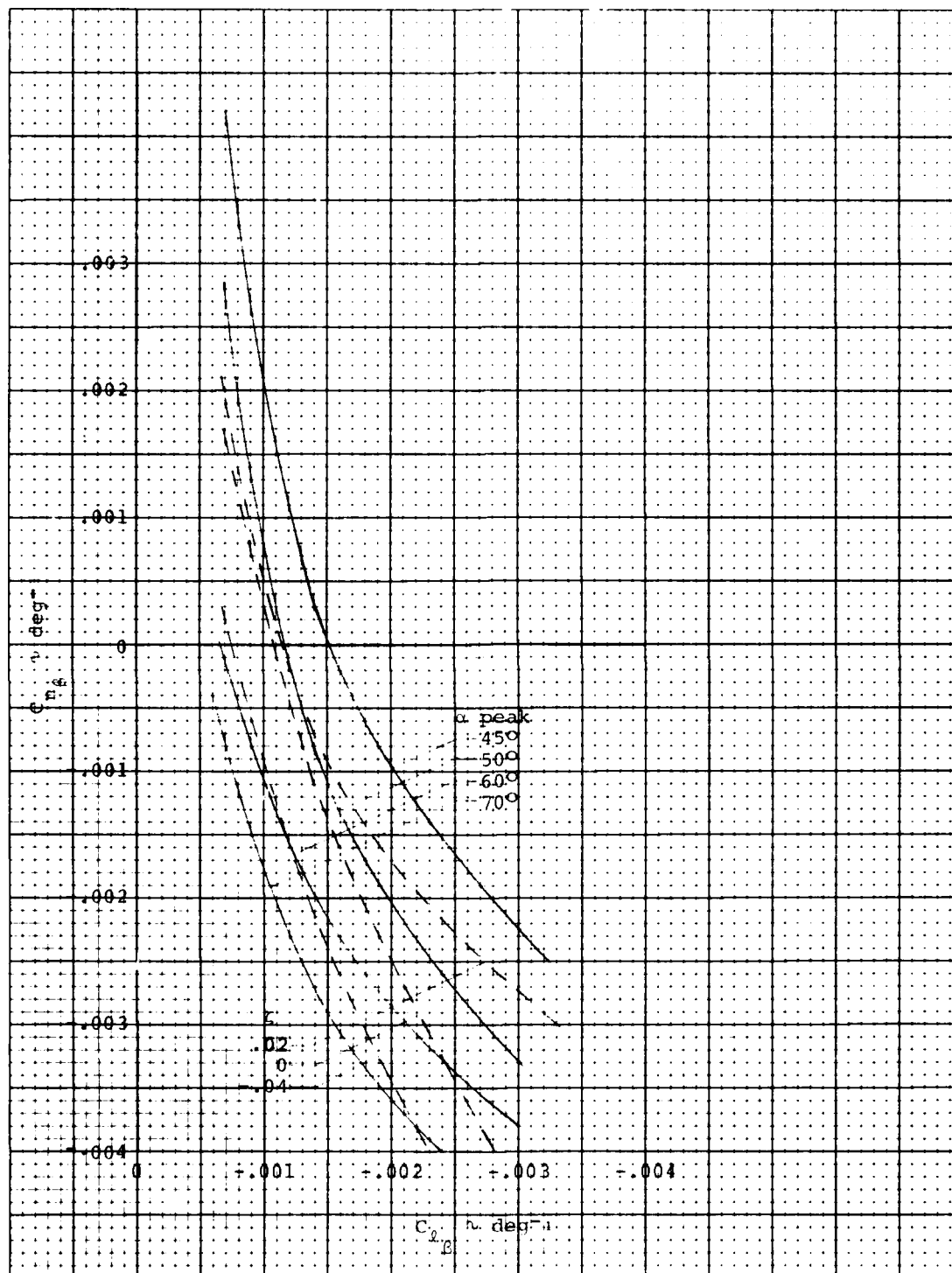
Figure 7. Constant \alpha peak and damping ratio curves as a function of lateral and directional stability for a 9% static margin airplane with proverse C_{n\beta}
