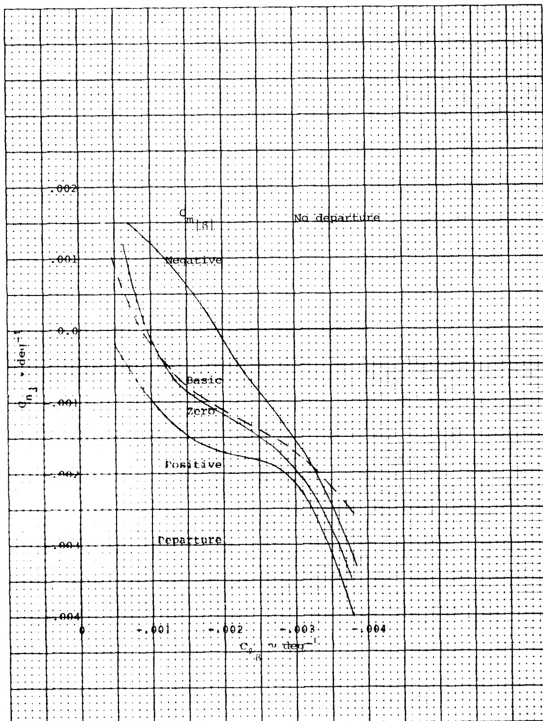
Figure 17. Influence of C_{m|\delta|} on departure boundaries for a 9% static margin airplane having adverse C_{n_{\delta}}
