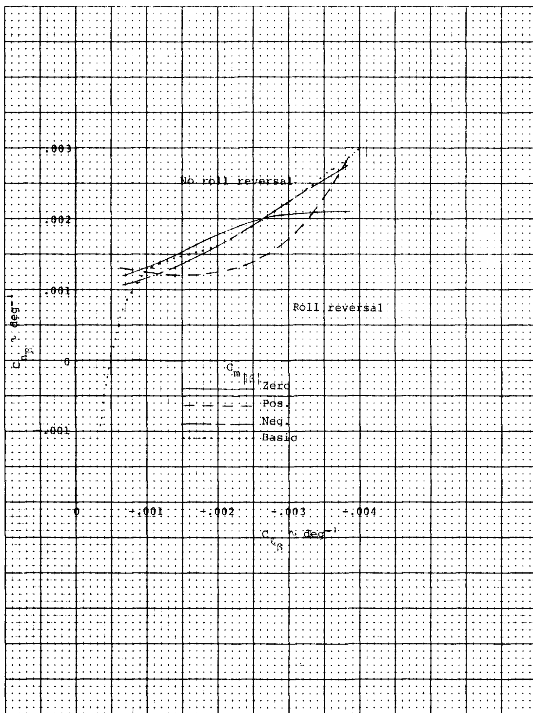
Figure 21. Influence of C_m on uncoordinated roll reversal boundaries for a 9% static margin airplane having adverse C_{n_{\delta a}}
