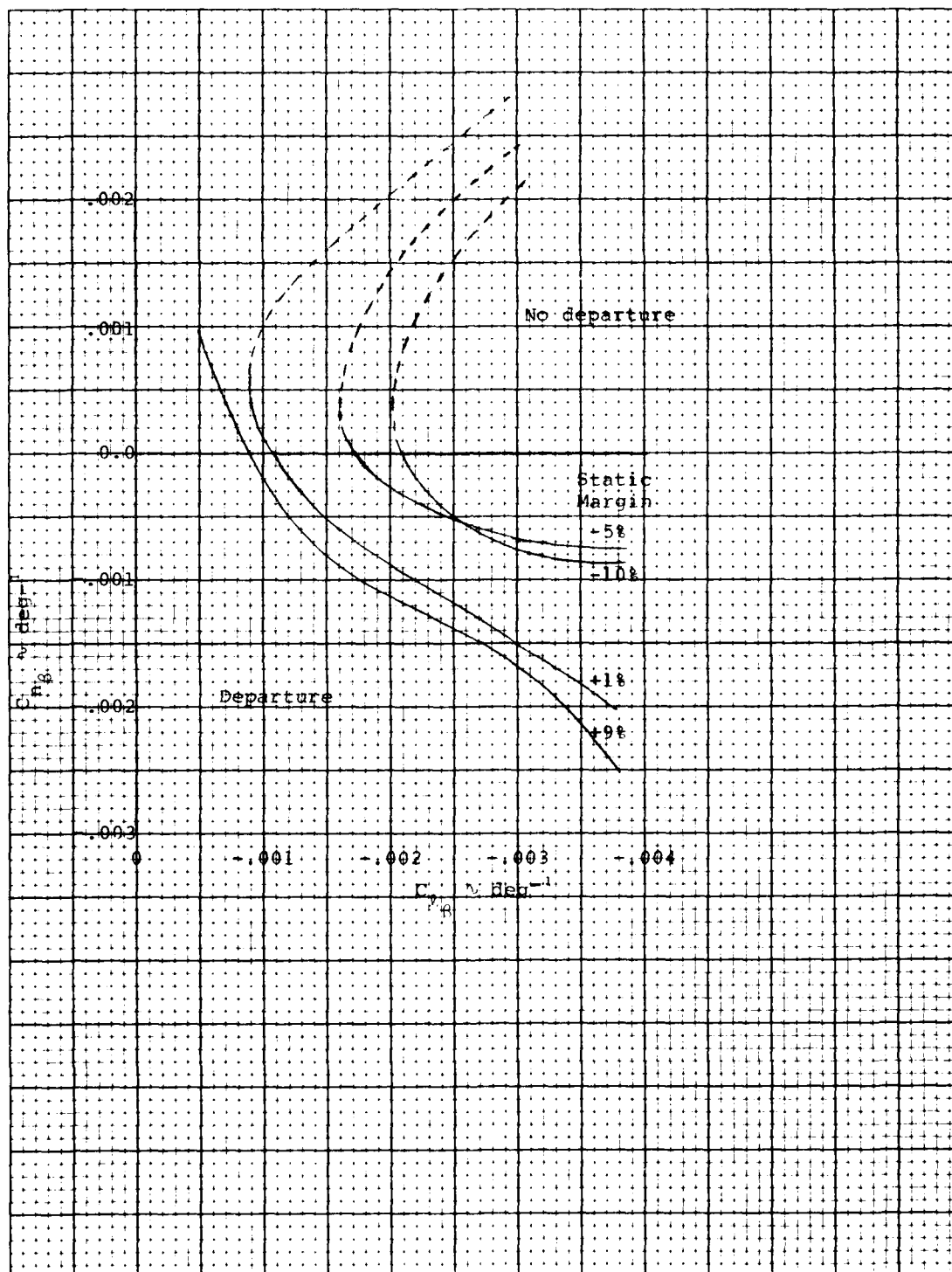
Figure 18. Influence of static margin on departure boundaries for augmented airplane having adverse C_{n\delta_a}
