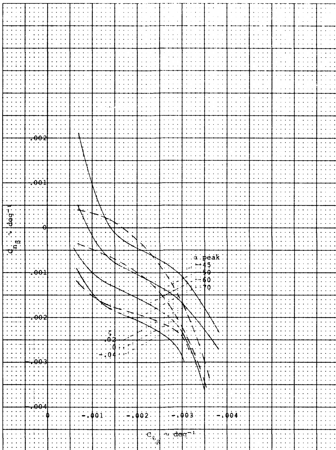
Figure 9. Constant alpha peak and damping ratio curves as a function of lateral and directional stability for 9° static margin airplane with adverse C_{n_{\dot{\alpha}}}
