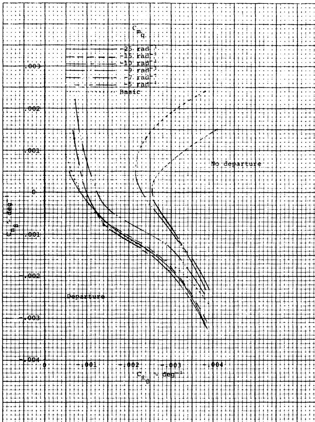
Figure 16. Influence of C_{mq} on departure boundaries for a 9% static margin airplane having adverse C_{n\beta a}
