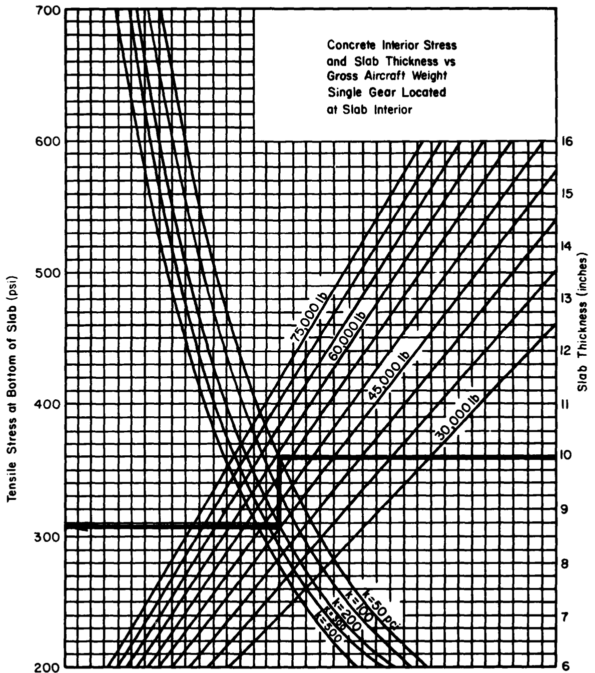
Figure 7. Chart for Obtaining the Tensile Stress at the Bottom of the Slab for a Single Wheel Gear Load.
