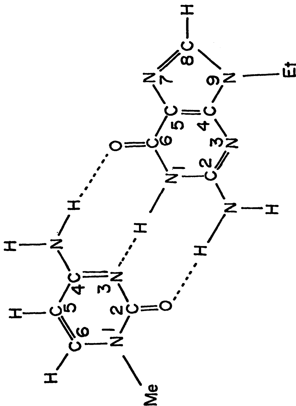
9-ethylguanine
