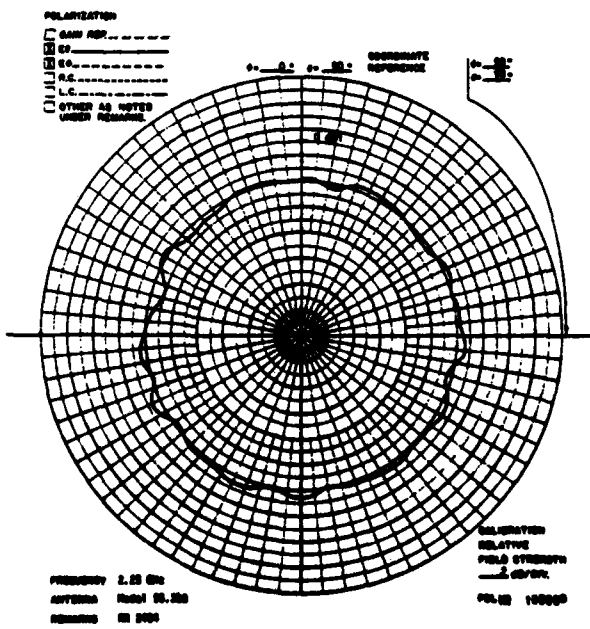
Figure 13. Roll Plane 48-Element Array
