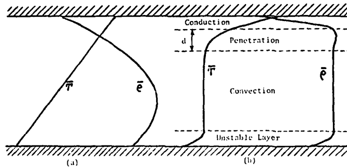
Fig. 1. Temperature and density profiles. (a) Conduction only. (b) Penetrative convection.
