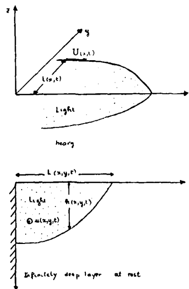
Fig. 2. Intrusion over an inactive deep layer.
