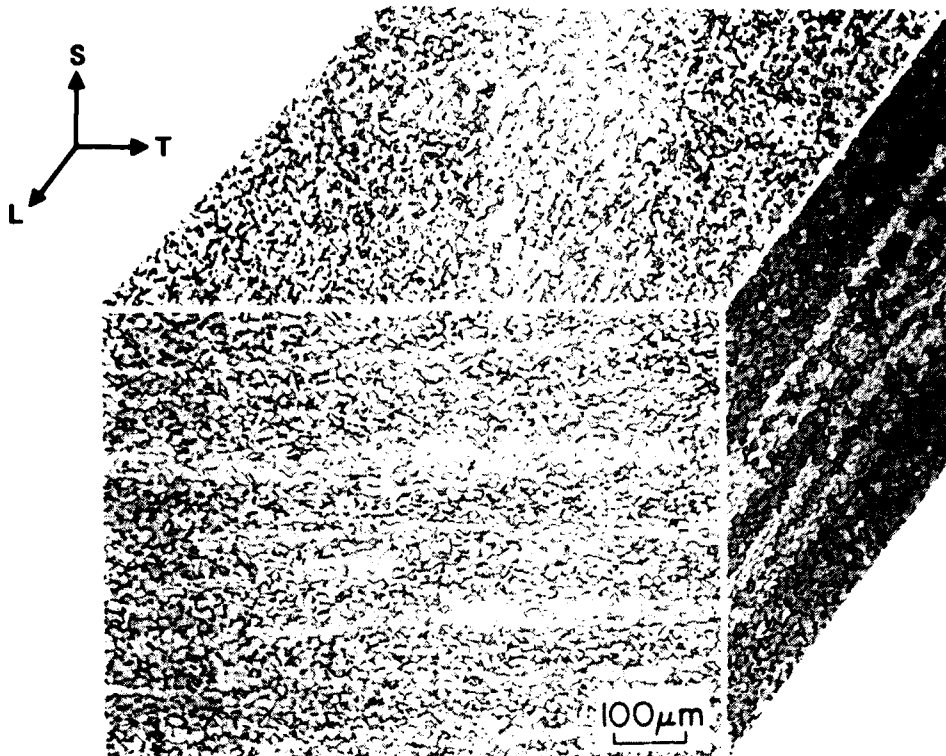
Fig. 1 Isometric view of Ti-6Al-4V used in this study. Note banding of primary alpha particles parallel to rolling plane.
