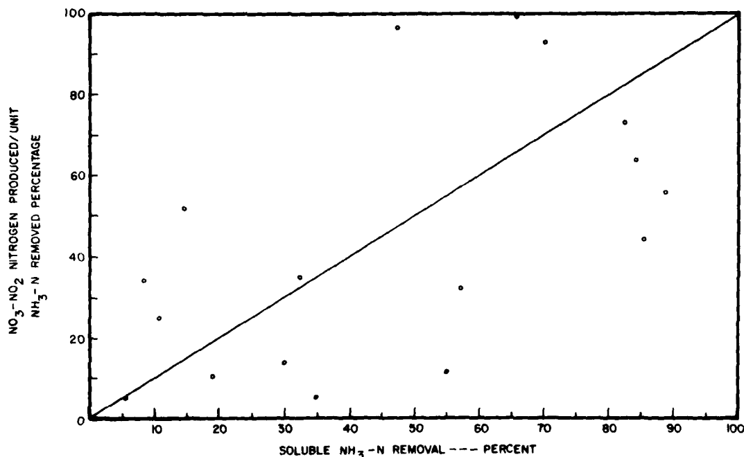
Figure 10. Soluble NH 3 -N removal at various loadings.
