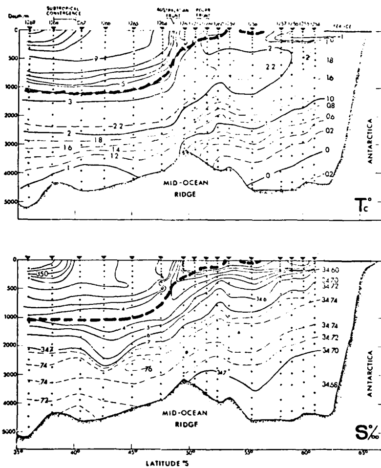
Fig. 6. Meridional temperature section along 115°E (from Gordon, Taylor and Georgi, 1977).
