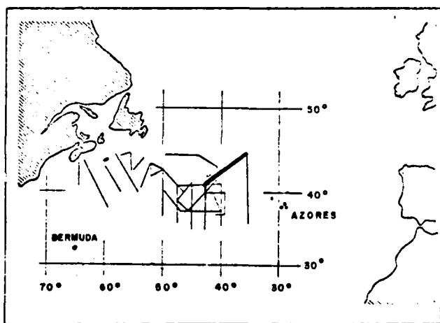
Fig. 3. CSS Baffin section off Newfoundland, showing 14°C water.
