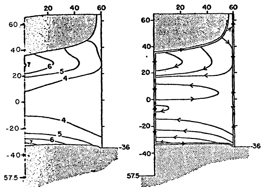
(left) Calculated thermocline depth (in hectometers) in Atlantic Ocean. Lower layer of surface in stippled regions. (right) Schematic of upper-layer transport for Atlantic.
