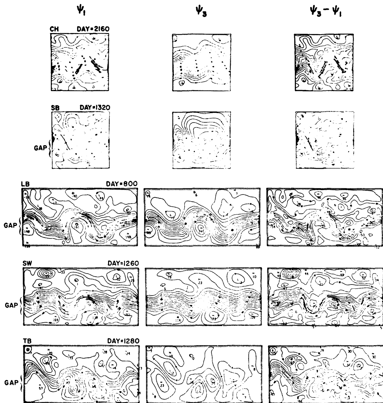
Fig. 7. Instantaneous streamfunction patterns on selected days during the equilibrium periods for the different cases. Shown for each case are the upper and lower streamfunctions and their difference, which, when multiplied by f_0/R' = -0.55 \cdot 10^{-2} \text{ s m}^{-1} , yields the interfacial displacement. The contour intervals are 10^4 \text{ m}^2 \text{ s}^{-1} for \psi_1 and 0.6 \cdot 10^3 \text{ m}^2 \text{ s}^{-1} for \psi_3 - \psi_1 ; the labels are in units of 10^3 \text{ m}^2 \text{ s}^{-1} . The range of \psi values in each of these figures (from left to right, top to bottom) is 292, 165, 132, 199, 105, 108, 205, 116, 103, 230, 126, 116, 117, 37, and 104 \cdot 10^3 \text{ m}^2 \text{ s}^{-1} , respectively.
