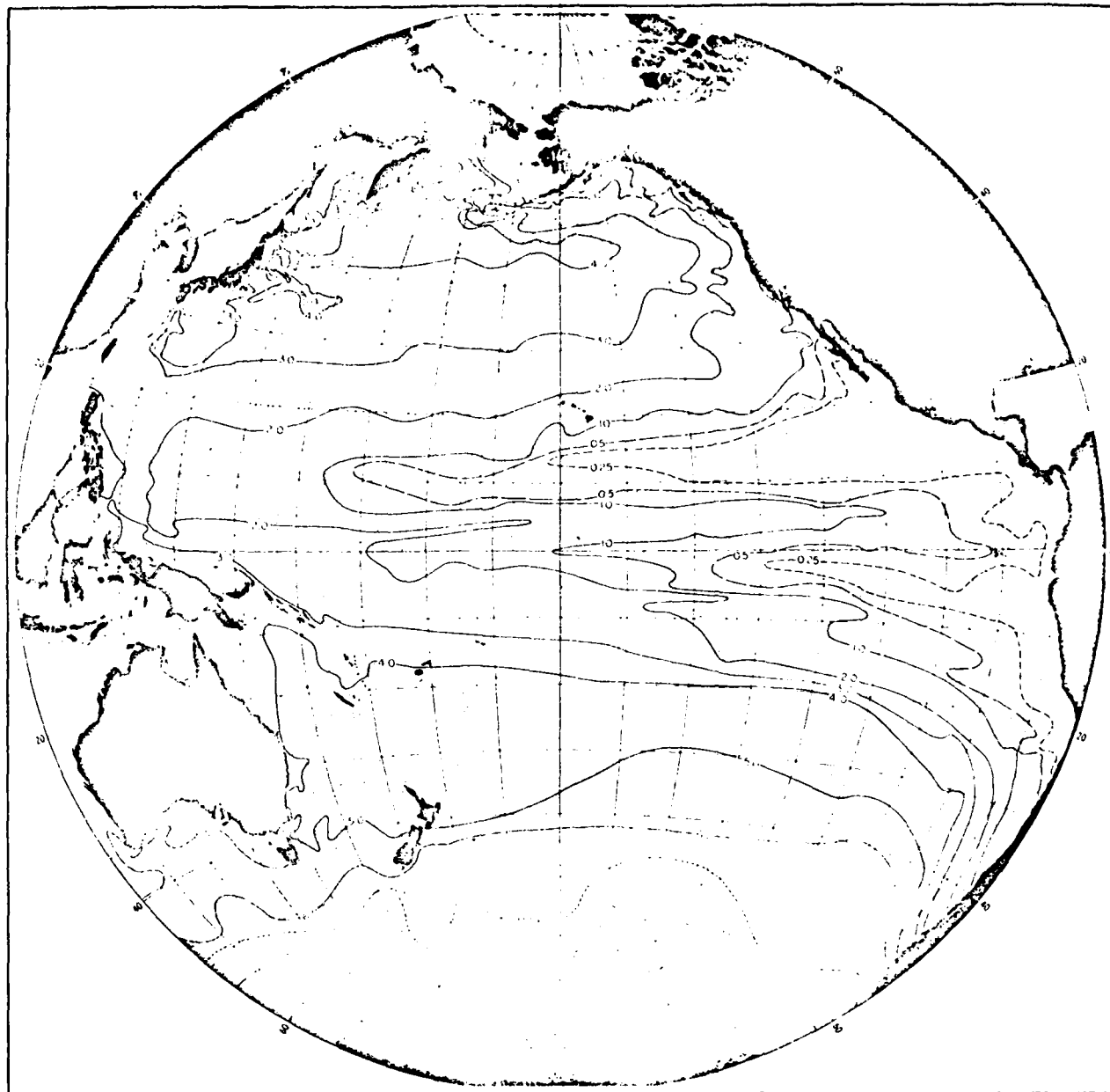
Fig. 2. Oxygen on \delta_T = 125 cl/ton in the Pacific Ocean (from Reid, 1965).
