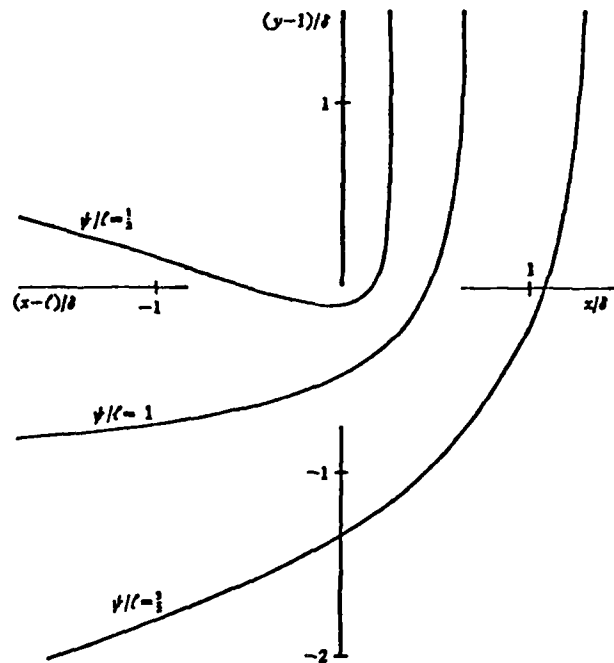
FIGURE 4. Transport lines, as given by (5.28), near the tip of the peninsula which corresponds in the model to Cape Horn. There is a transport of 2a_0 which goes into a 'western boundary current' seen here to the right of the diagram. There is no exaggeration of the north-south scale.
