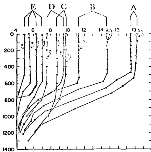
Fig. 10. Representative Late winter stations from the North Atlantic.
