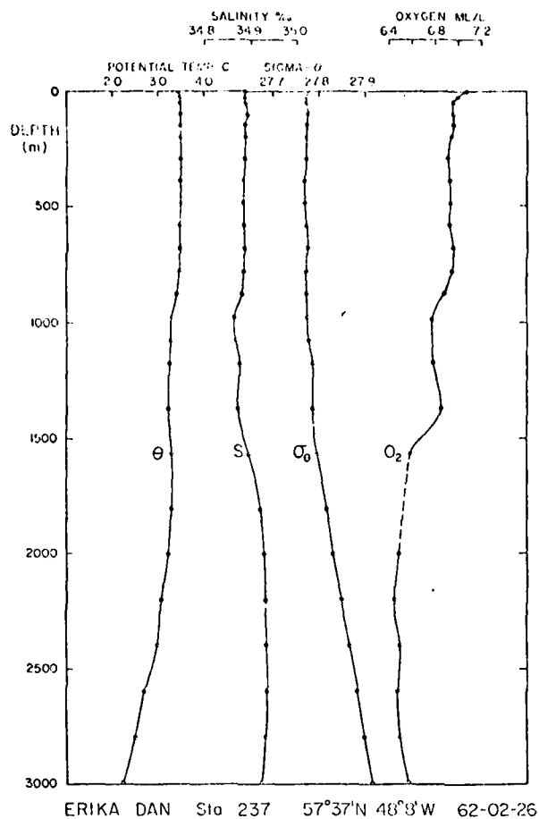
Fig. 11. Sounding in Labrador Sea indicating deep mixing.
