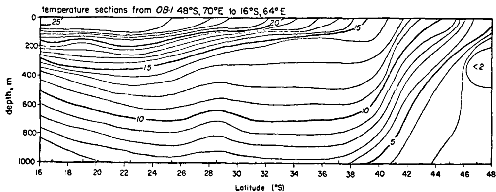
Fig. 12. Southern Ocean temperature section from OE-1 .
