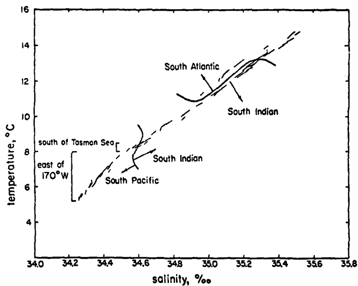
Fig. 18. T-S curves for SAMW capped below summer thermoclines.
