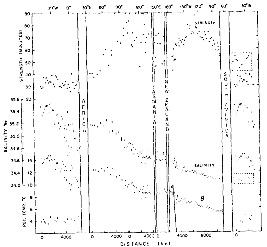
Fig. 1. Variations of AAIW properties around Antarctica.
