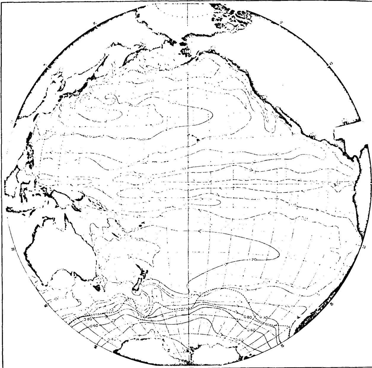
Fig. 3. Acceleration potential for \delta_T=125 cl/ton relative to 2000 db (from Reid, 1965).
