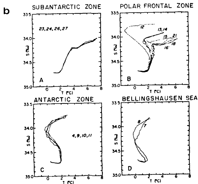
Fig. 8b. \theta -S curves from the various zones from 60-68°W across Drake Passage (ibid.).
