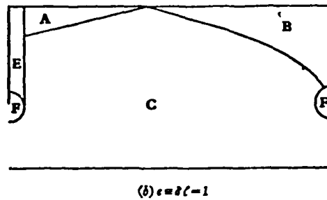
FIGURE 3. A schematic picture of the boundary layers that exist when the friction parameter \delta is small. (a) is the case where the product \delta l is also small, (b) the case where \delta l is of order unity. The layers E and F are of thickness \delta while A and C have average thickness of order (\delta l)^{\frac{1}{2}} . The Sverdrup (or in case (b) the modified Sverdrup) solution is valid in B while the zonal solution is valid in D. The western boundary current flows in E. The behaviour of the transport lines in F is shown in figure 4.
