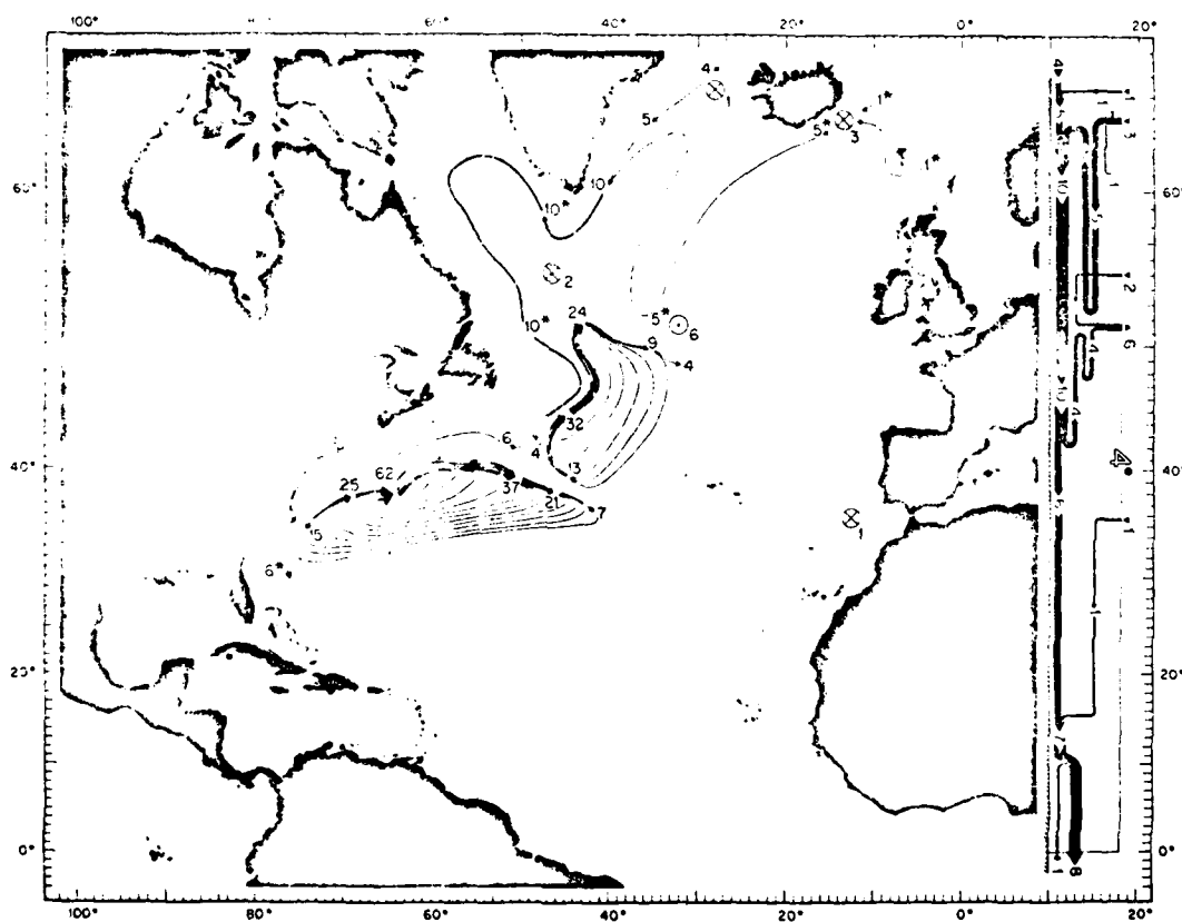
Fig. 2. Circulation diagram and box model for the deep ( \theta < 4.0^\circ\text{C} ) circulation in the North Atlantic (Worthington, 1976, Fig. 11).
