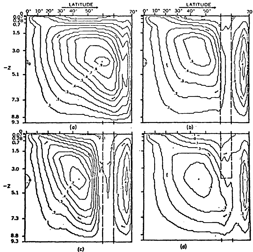
Fig. 6. Meridional circulation in the model ocean for cases (a) 14-I (closed basin), (b) 15-I (deep gap, linear surface-temperature distribution), (c) 16-I (deep gap, curved surface-temperature distribution), and (d) 18-I (shallow gap, linear surface-temperature distribution). Contours of the mass transport stream function, \psi^{(m)} , are shown in non-dimensional units. \psi^{(m)} is zero on the boundaries.
