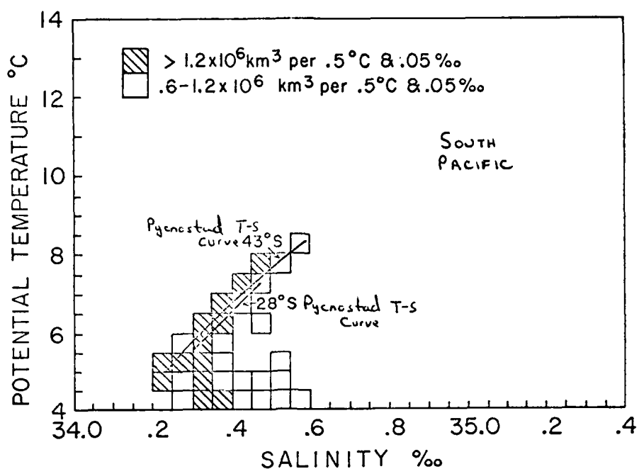
Fig. 19. Volumetric T-S diagram for the South Pacific.
