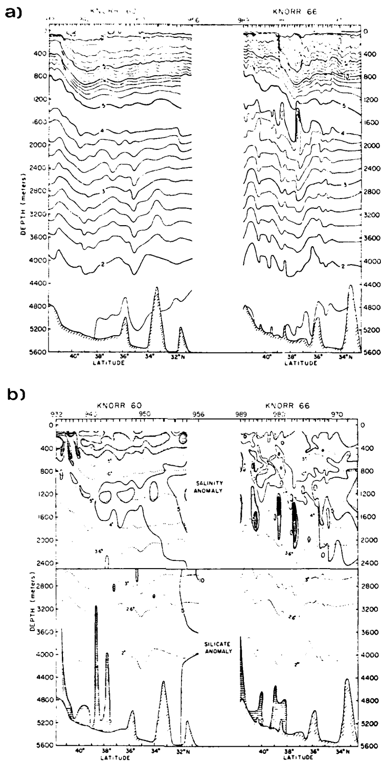
Fig. 3. Comparison of sections along 55^{\circ}\text{W} in October 1976 and August 1977. a) Potential temperature. b) Salinity anomaly ( Z < 2500\text{m} ) and silicate anomaly ( Z > 2500\text{m} ). (McCartney, Worthington and Raymer, 1979).
