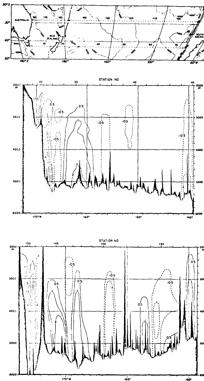
Fig. 4. Sections showing existence of western intensified deep motion boundary currents in the South Pacific Ocean (Warren, 1973).
