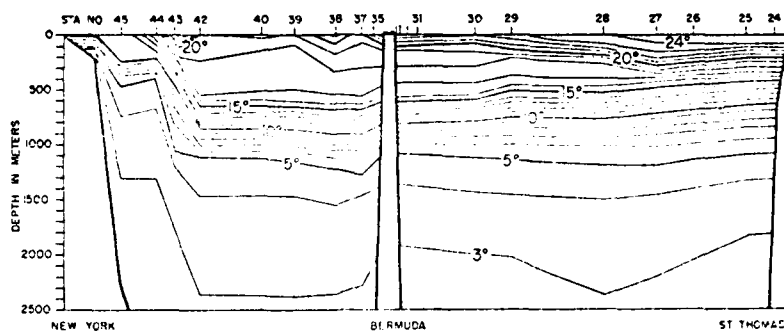
Fig. 3. The Eighteen Degree Water thermostad of the Sargasso Sea as discovered by the CHALLENGER Expedition in 1873. (Worthington, 1976, Fig. 32).
