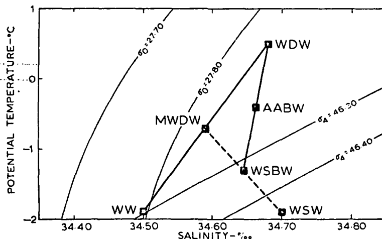
Fig. 1. Mixing Processes Leading to Antarctic Bottom Water (AABW), WW = Winter Water, WDW = Warm Deep Water, WSW = Western Shelf Water, MWDW = Modified Warm Deep Water, WSBW = Weddell Sea Bottom Water.
