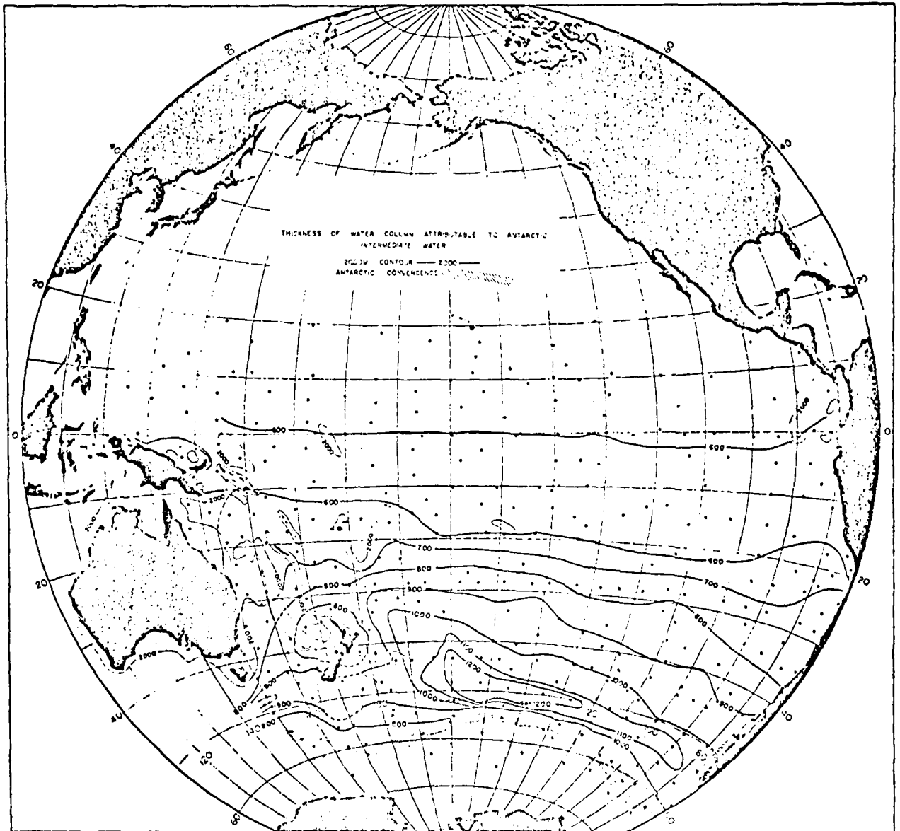
Fig. 3. AAIW equivalent thickness.
