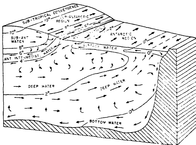
Fig. 6. An example of Sverdrup's (1933) technique of inference of meridional flow components from core layers.
