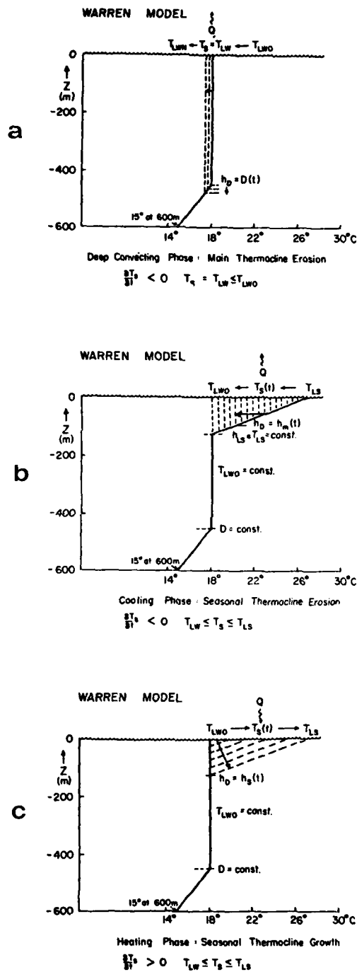
Fig. 9. Temperature structure changes during the three phases of Warren's (1972) local formation model for Eighteen Degree Water.
