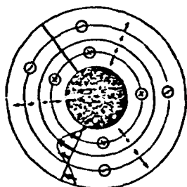
a. The schematic Southern Ocean. Antarctica is the solid, black circle. The meridional barrier extending northward from Antarctica is represented by the solid heavy black vertical line. The schematic wind system (purely zonal) is depicted by the heavy arrows on the lower left. The concentric circles are latitude circles. Latitudes of EKMAN convergence and sinking at the surface are indicated by minus signs, latitudes of EKMAN divergence and upwelling are indicated by plus signs. The direction of the required meridional geostrophic flow is indicated by light radial arrows.
