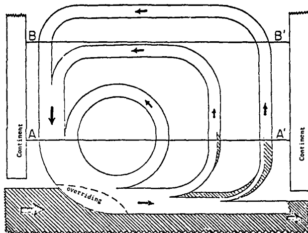
Fig. 9. Schematic anticyclonic circulation in the southern oceans.
