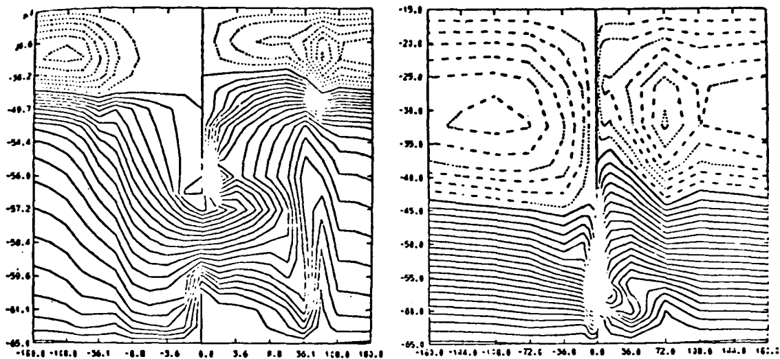
Streamlines for Scotia Ridge topography, \delta = 0.1 , R_0 = 0 , H = 3 for \lambda \geq 35^\circ , \theta = -56.5^\circ , -61^\circ ; H = 1 at \lambda = 35^\circ , -61.0^\circ \leq \theta \leq -56.5^\circ ; H = 5 elsewhere. Transport = 90 Sverdrups.
