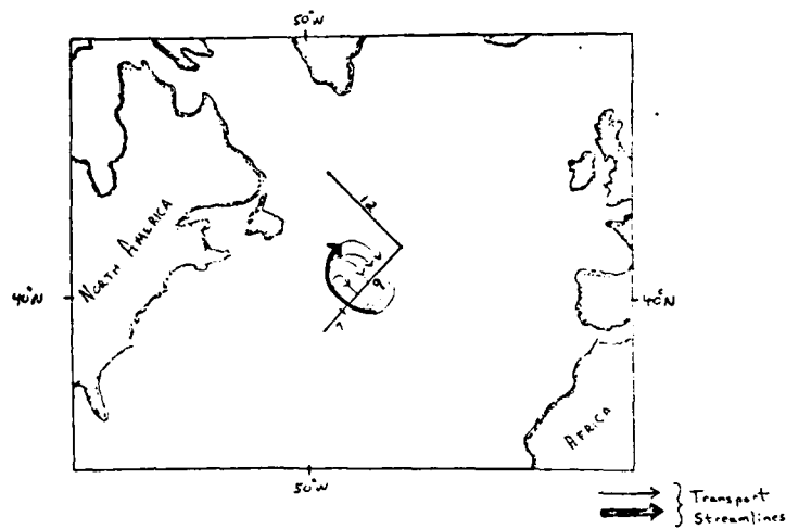
Fig. 4. Location map for sections 7, 9 and 12, showing Worthington's (1976) Northern Gyre.
