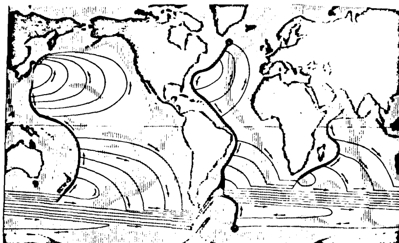
Fig. 1. Schematic theoretical pattern of deep circulation in the world ocean (Stommel, 1958).
