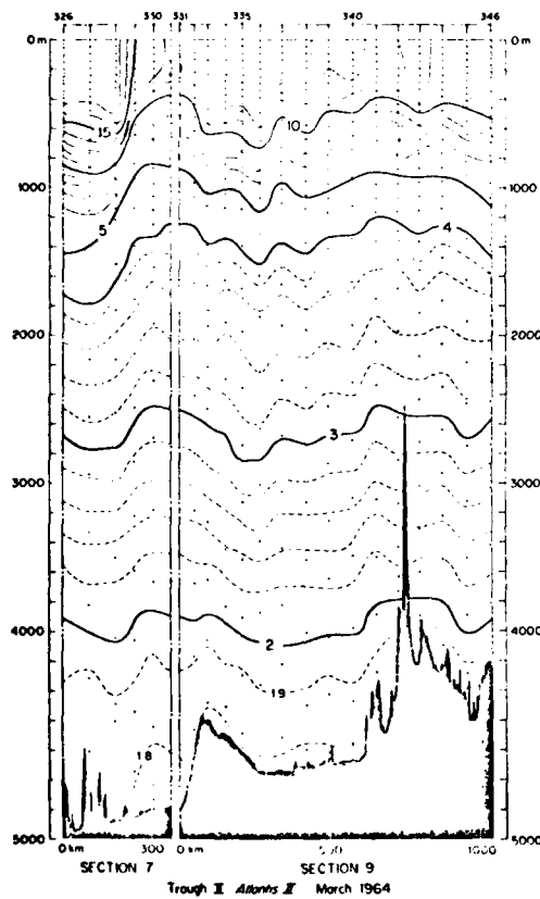
Fig. 5. Temperature sections 7 and 9.
