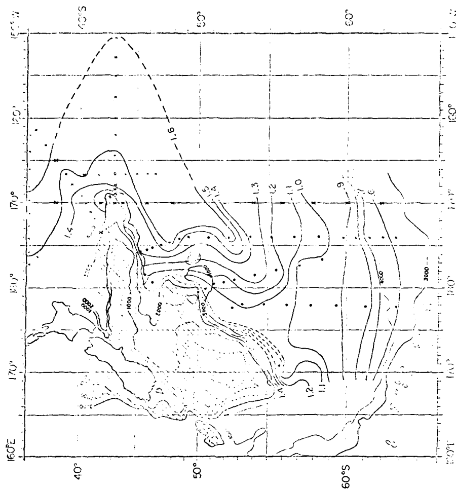
Fig. 2. Horizontal temperature distribution on the 3000 db pressure surface off New Zealand.
