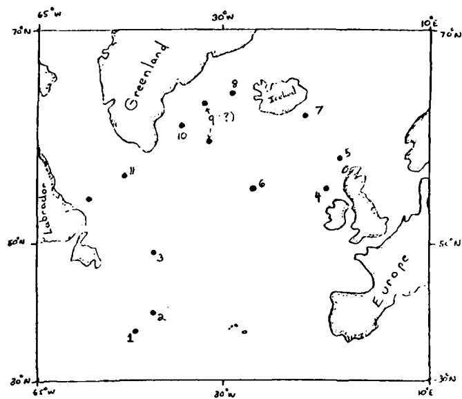
Fig. 9. Location of Late Winter North Atlantic stations.
