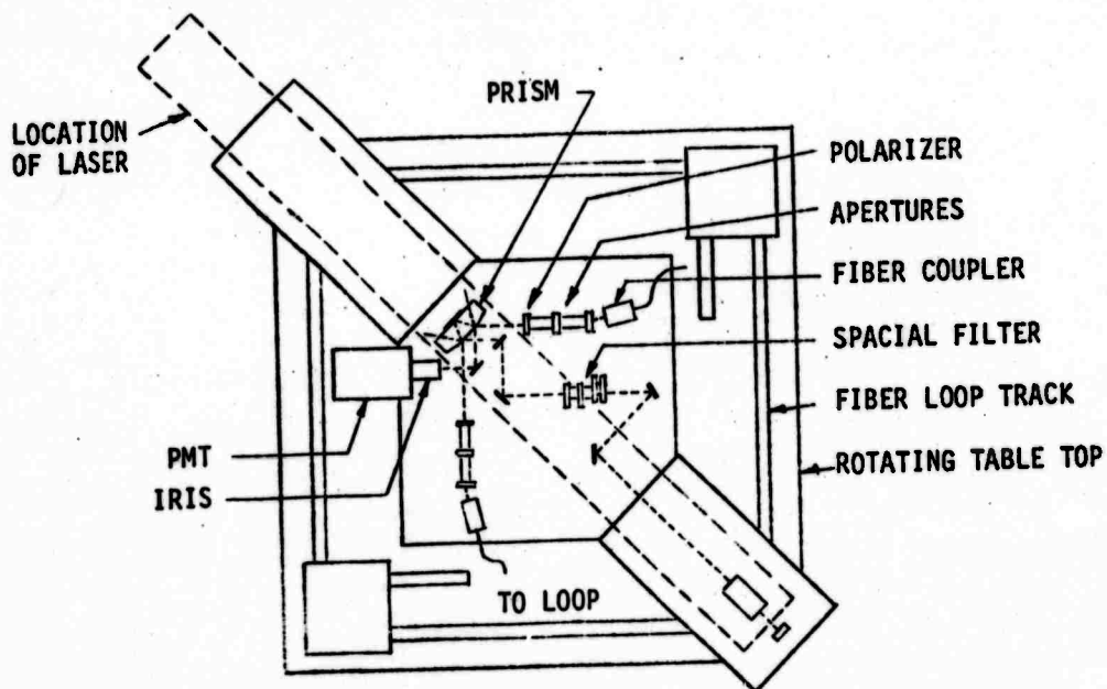
FIG. 9--Experimental system.
