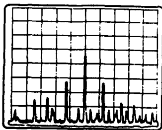
OUTPUT SPECTRUM CENTER FREQUENCY: 7.8 GHz
