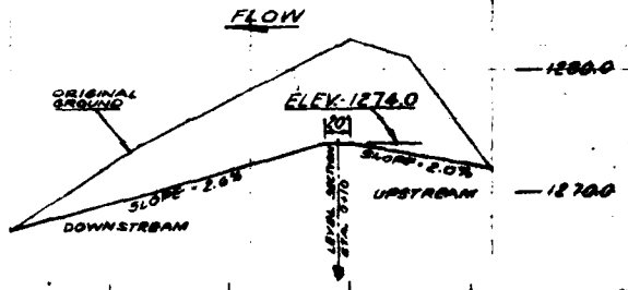
PROFILE ALONG E OF EMERGENCY SPILLWAY SCALE: HORIZONTAL: 1"=80' VERTICAL: 1"=8'
