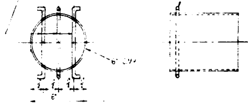
DETAIL OF SMALL ANIMAL GUARD - NOT TO SCALE (1 REQ.)
