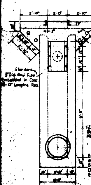
REAR ELEVATION
