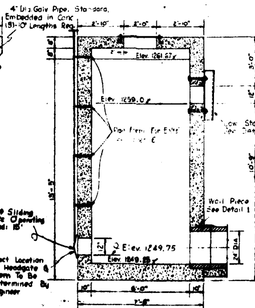
SECTION ON CENTERLINE
