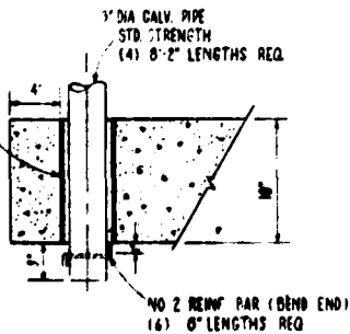
SECTION AA SCALE 1/4"=1'
