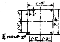
STEEL COVER PLATE (1/4" THICK)
