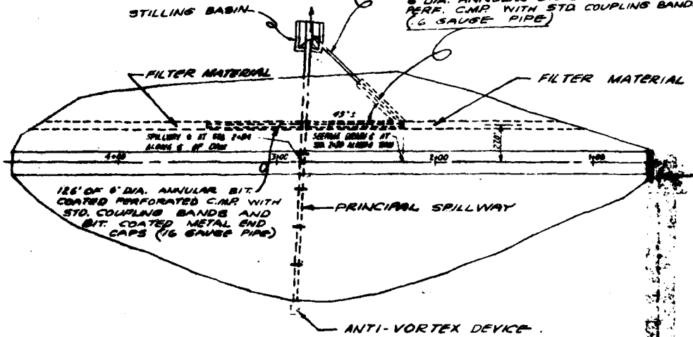
PLAN VIEW OF SEEPAGE & TOE DRAIN SCALE: 1"=40'
