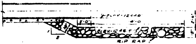
SECTION ON CENTERLINE
