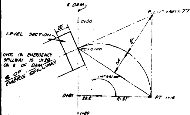
LAYOUT OF EMERGENCY SPILLWAY CURVE SCALE: 1" = 30'
