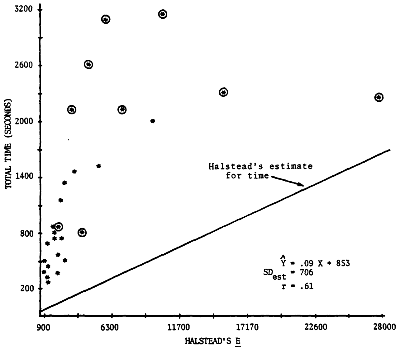
Figure 4. Scatterplot of Halstead's E with total time
