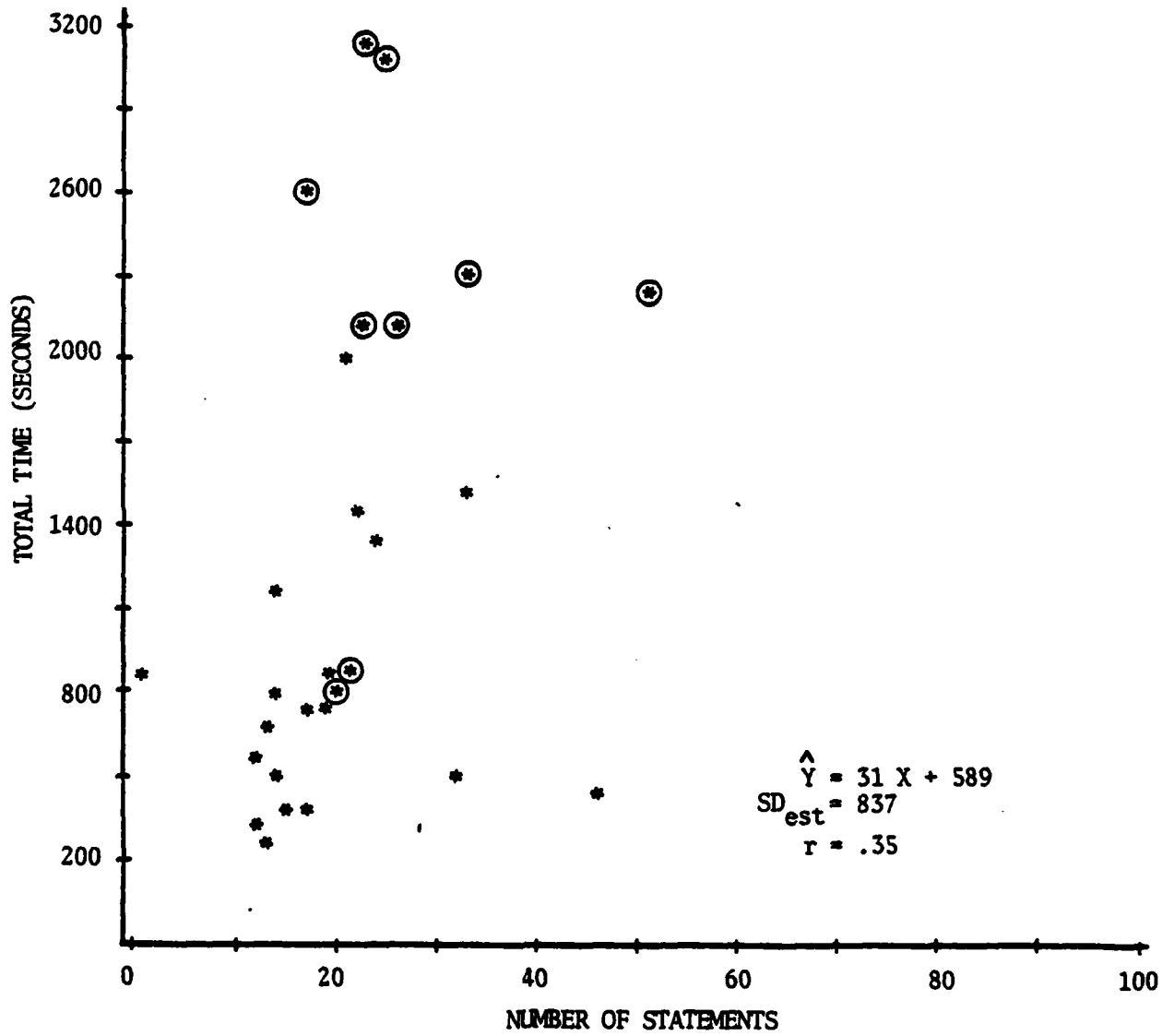
Figure 2. Scatterplot of number of statements with total time
