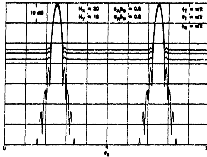
Figure 7. Equispaced Planar Array, Hanning Weights, \phi_1 = \pi/2 , \theta_1 = \pi/2 , \phi_2 = \pi/2 , Q = .1 , \sigma_T^2 = .1 , \sigma_\theta^2 = .1
