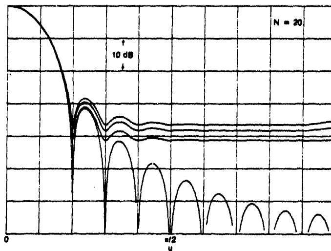
Figure 3B. Q = 0 , \sigma_r^2 = .001 , \sigma_p^2 = 0
