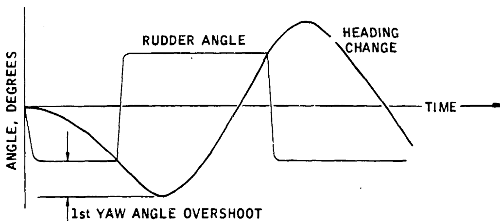
FIGURE 4. DEFINITION DIAGRAMS
