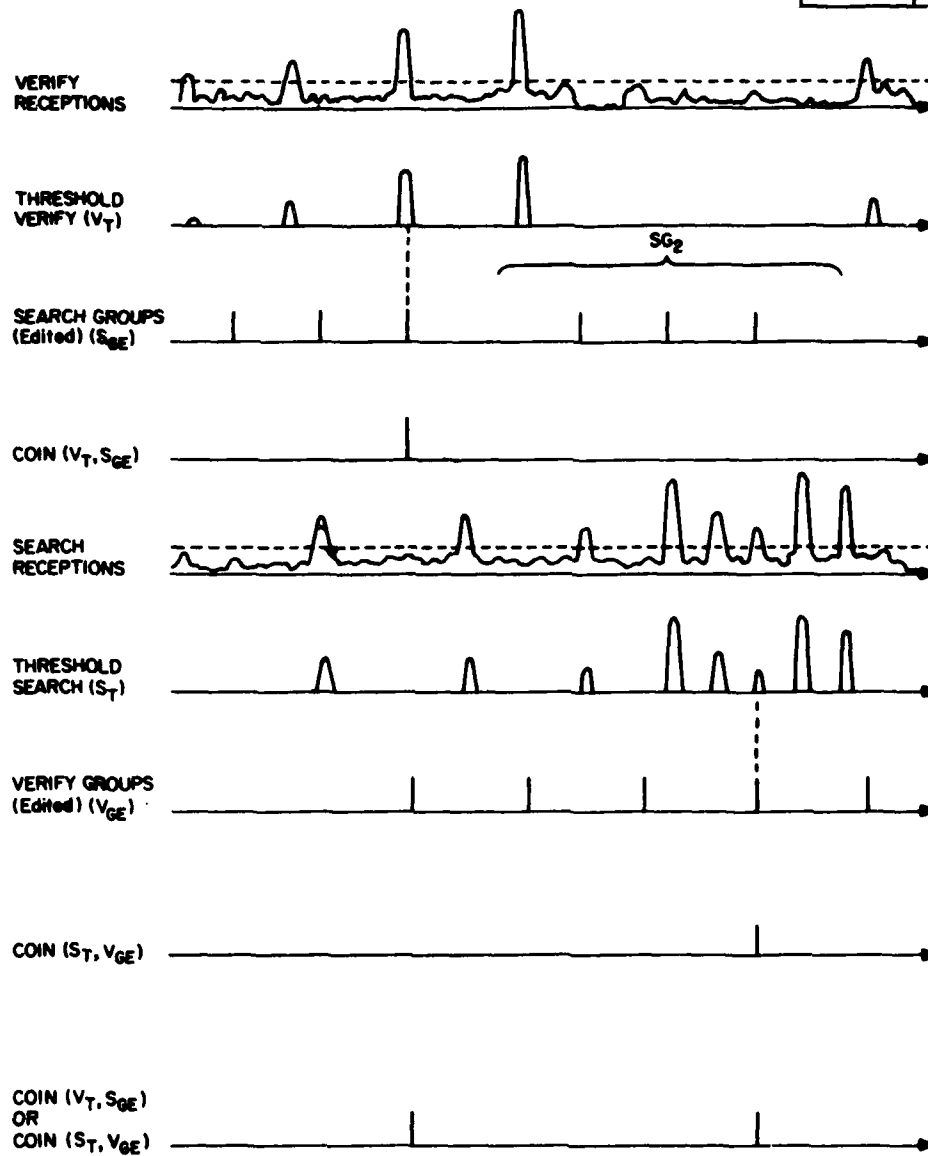
Fig. 4c. Bulk filter - coincidence.
