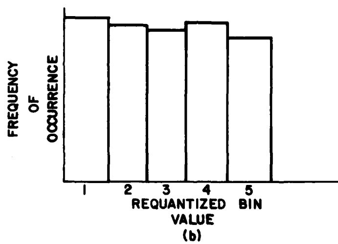
Fig. 6. Histogram equalization.
