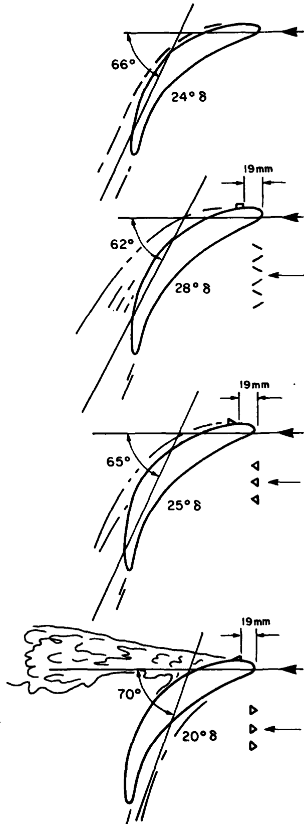
FIG. A-4: STATIC TESTS (VORTEX GENERATORS)
