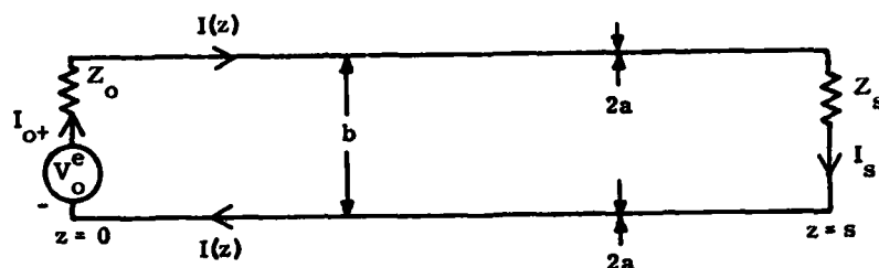
Figure 1. Transmission Line Terminated in Load Impedances Z_o and Z_s and Driven by Voltage V_o^e .
