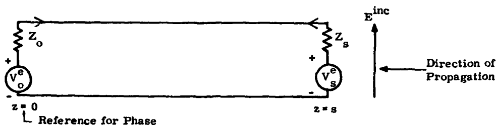
Figure 3. Diagram for Determining the Current in the Load Impedances of a Transmission Line Driven by Generators V_o^e and V_s^e .
