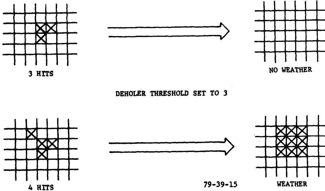
FIGURE 15. DEHOLER OPERATION
