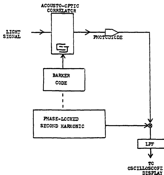
Fig.3.16 Electronic Arrangement for Barker Code Detection
