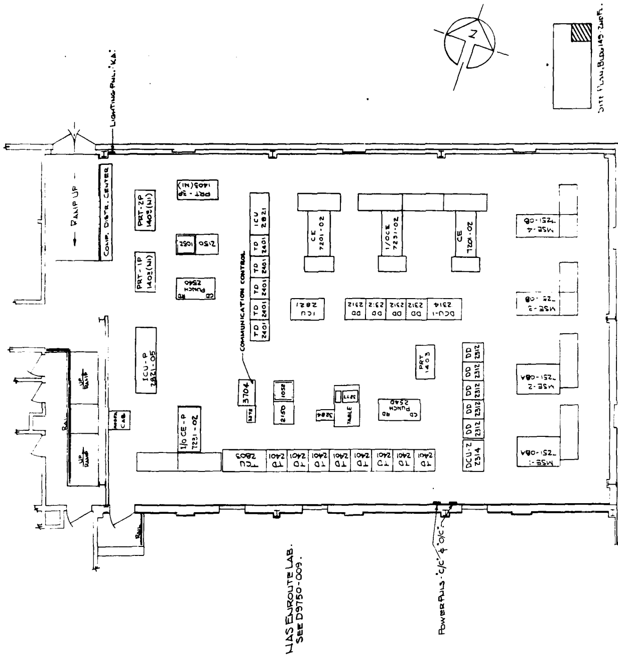
FIGURE A-7 JOBSHOP ROOM LAYOUT
