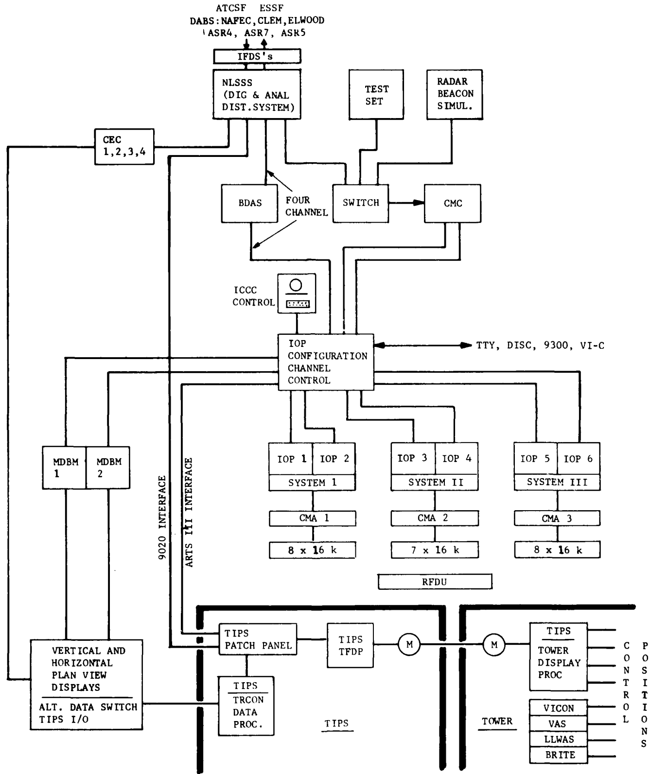
FIGURE 2-12 PROPOSED TATF SYSTEM CONFIGURATIONS
