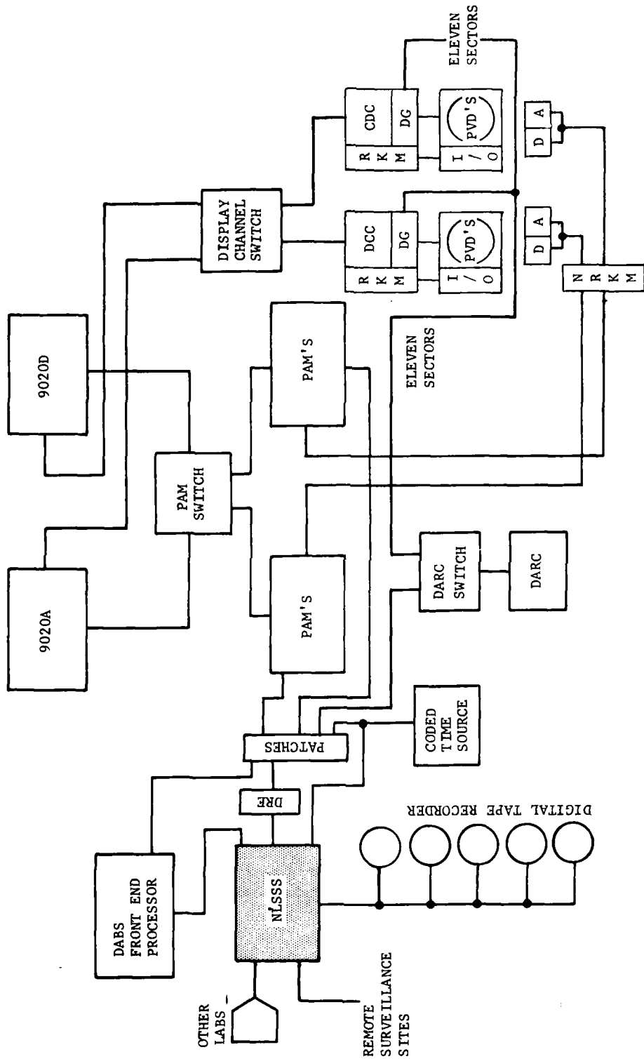
FIGURE 2-5 ESSF WITH NLSS INCLUDED
