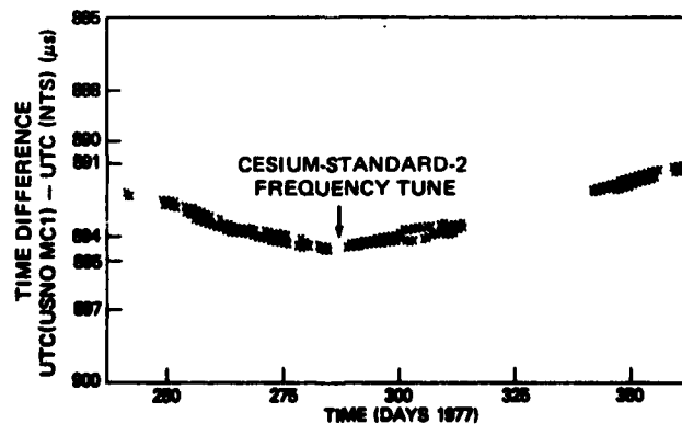
Fig. 13 — Clock differences between UTC(NTS) via the Panama station and UTC(USNO, MC1)
