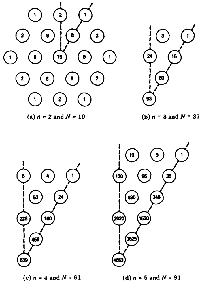
Fig. 7 — Array excitations for n = 2 through 5 for a = 1/3
