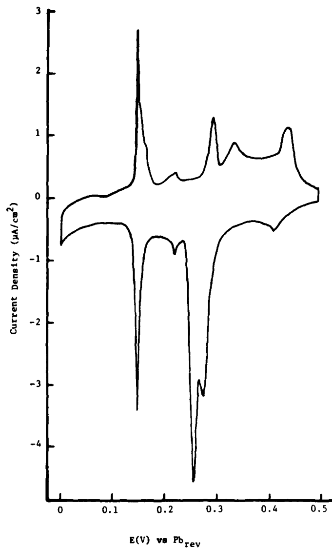
Figure 5.10 Voltammogram for the UPD of Pb on Au(100)-(5x20) in 0.1 M HF + 1mM Pb (NO 3 ) 2 . Sweep rate: 2 mV/s. Initial Potential: 0.0V.
