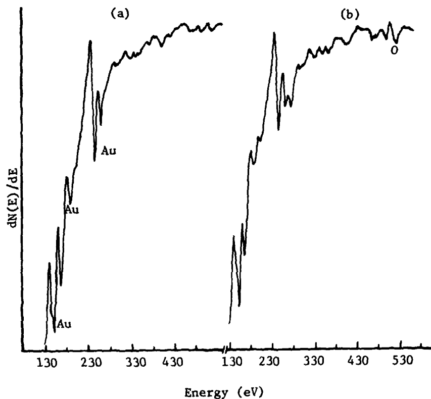
Figure 5.18 a. Auger spectrum of a clean Au(100) single crystal. Beam energy: 1800 eV. Beam current: 13 \mu A. Modulation voltage: 10 V. b. Same surface and conditions as a except crystal subjected to electrochemical treatment. The electrode was initialized at 0.0 V and cycled approximately 20 times between 0 and 0.7 V. It was removed from the thin-layer cell at 50 mV on the cathodic sweep.
